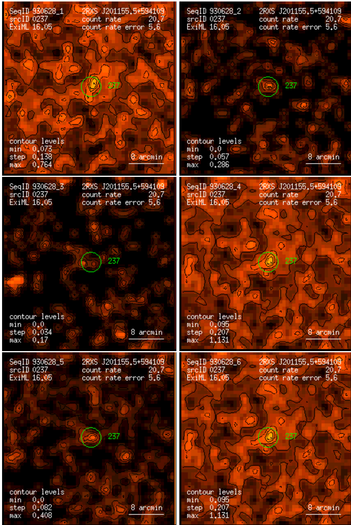
Figure 237: RASS 930628: detection 0237: band rate images, Gaussian filter: (1) PSPC channels 11 – 41, (2) 52 – 90, (3) 91 – 201, (4) 11 – 235, (5) 52 – 201, (6) 11 – 201. Broad band rates in counts/ks. Band rate contour levels in counts/ks/arcmin 2 .
