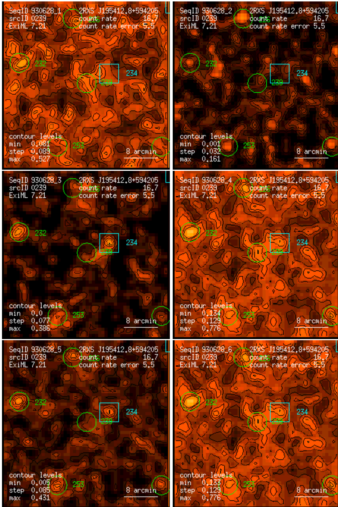
Figure 239: RASS 930628: detection 0239: band rate images, Gaussian filter: (1) PSPC channels 11 – 41, (2) 52 – 90, (3) 91 – 201, (4) 11 – 235, (5) 52 – 201, (6) 11 – 201. Broad band rates in counts/ks. Band rate contour levels in counts/ks/arcmin 2 .
