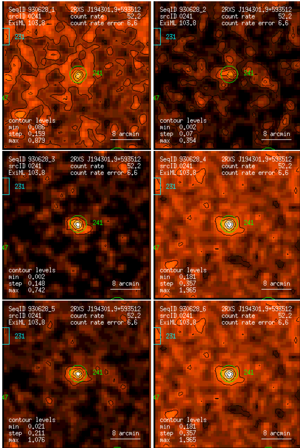
Figure 241: RASS 930628: detection 0241: band rate images, Gaussian filter: (1) PSPC channels 11 – 41, (2) 52 – 90, (3) 91 – 201, (4) 11 – 235, (5) 52 – 201, (6) 11 – 201. Broad band rates in counts/ks. Band rate contour levels in counts/ks/arcmin 2 .
