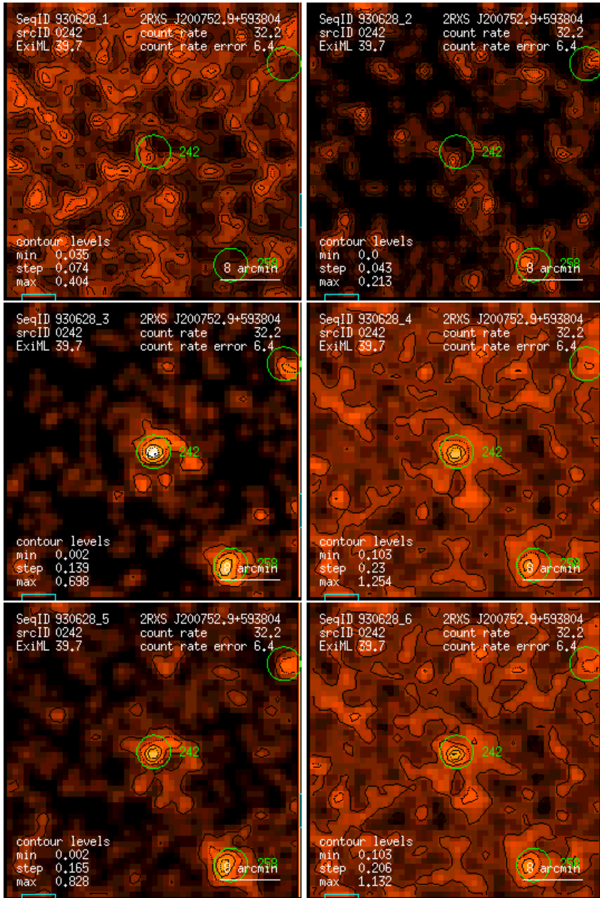
Figure 242: RASS 930628: detection 0242: band rate images, Gaussian filter: (1) PSPC channels 11 – 41, (2) 52 – 90, (3) 91 – 201, (4) 11 – 235, (5) 52 – 201, (6) 11 – 201. Broad band rates in counts/ks. Band rate contour levels in counts/ks/arcmin 2 .
