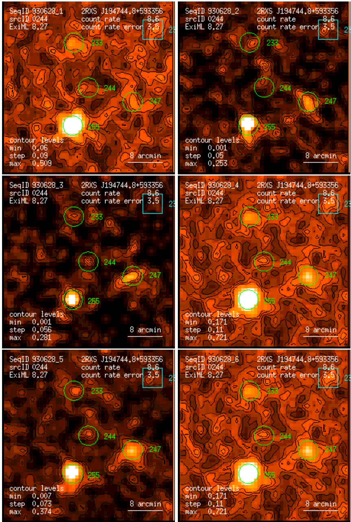
Figure 244: RASS 930628: detection 0244: band rate images, Gaussian filter: (1) PSPC channels 11 – 41, (2) 52 – 90, (3) 91 – 201, (4) 11 – 235, (5) 52 – 201, (6) 11 – 201. Broad band rates in counts/ks. Band rate contour levels in counts/ks/arcmin 2 .
