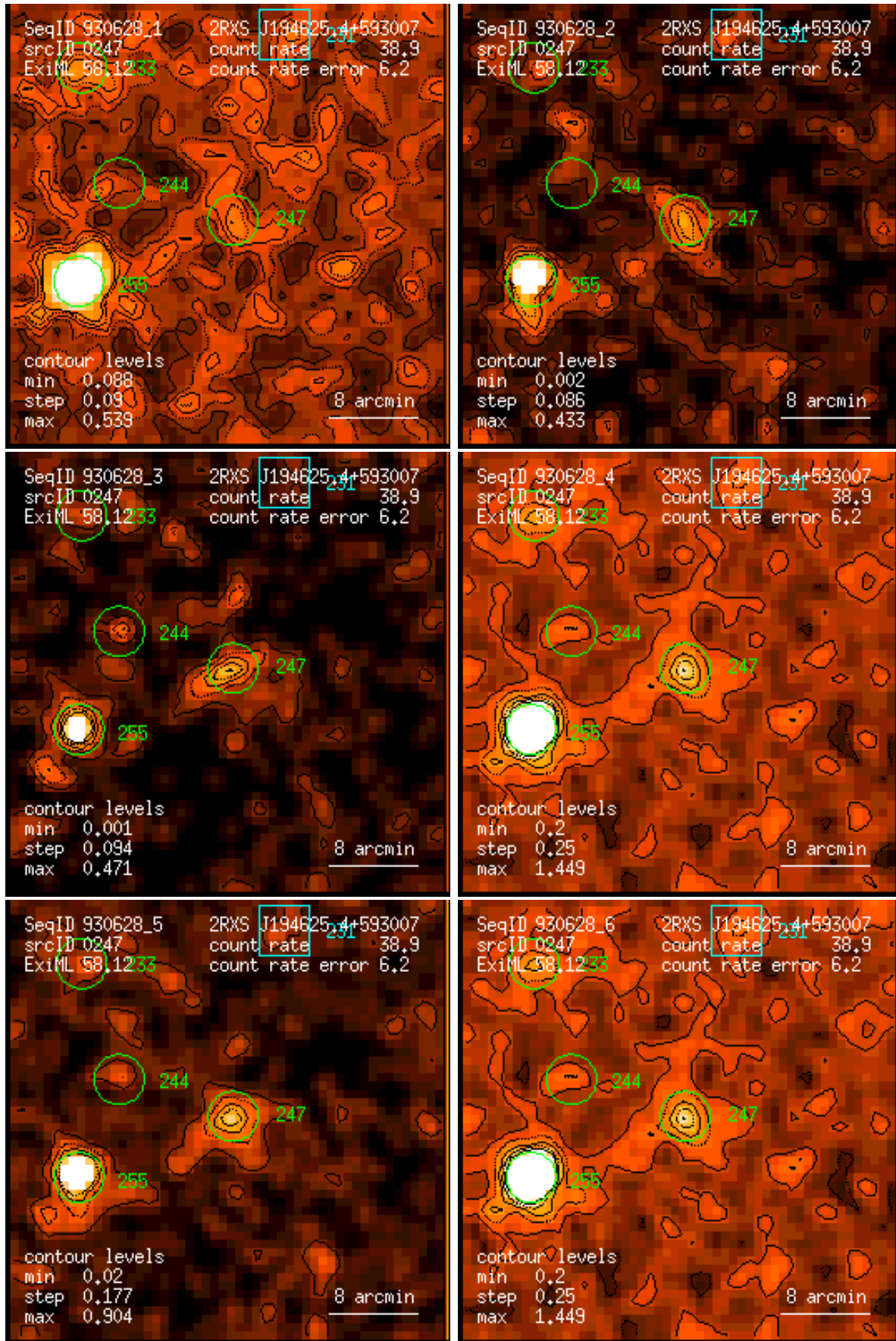
Figure 247: RASS 930628: detection 0247: band rate images, Gaussian filter: (1) PSPC channels 11 – 41, (2) 52 – 90, (3) 91 – 201, (4) 11 – 235, (5) 52 – 201, (6) 11 – 201. Broad band rates in counts/ks. Band rate contour levels in counts/ks/arcmin 2 .
