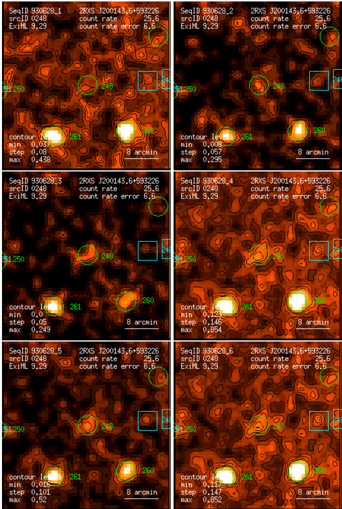
Figure 248: RASS 930628: detection 0248: band rate images, Gaussian filter: (1) PSPC channels 11 – 41, (2) 52 – 90, (3) 91 – 201, (4) 11 – 235, (5) 52 – 201, (6) 11 – 201. Broad band rates in counts/ks. Band rate contour levels in counts/ks/arcmin 2 .
