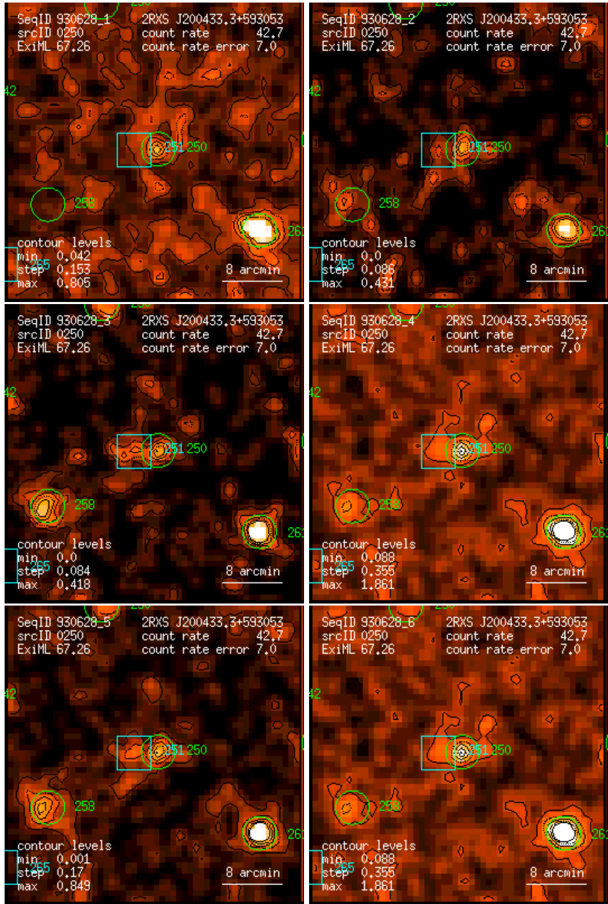
Figure 250: RASS 930628: detection 0250: band rate images, Gaussian filter: (1) PSPC channels 11 – 41, (2) 52 – 90, (3) 91 – 201, (4) 11 – 235, (5) 52 – 201, (6) 11 – 201. Broad band rates in counts/ks. Band rate contour levels in counts/ks/arcmin 2 .
