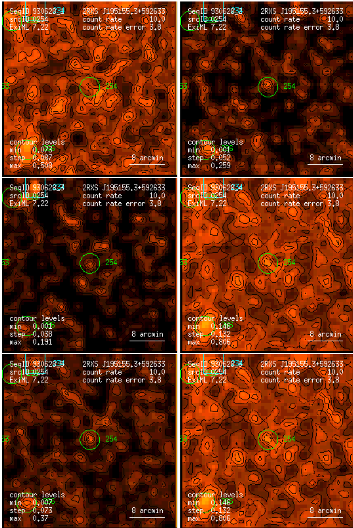
Figure 254: RASS 930628: detection 0254: band rate images, Gaussian filter: (1) PSPC channels 11 – 41, (2) 52 – 90, (3) 91 – 201, (4) 11 – 235, (5) 52 – 201, (6) 11 – 201. Broad band rates in counts/ks. Band rate contour levels in counts/ks/arcmin 2 .
