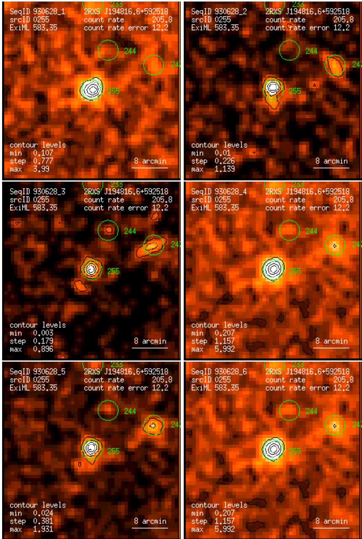
Figure 255: RASS 930628: detection 0255: band rate images, Gaussian filter: (1) PSPC channels 11 – 41, (2) 52 – 90, (3) 91 – 201, (4) 11 – 235, (5) 52 – 201, (6) 11 – 201. Broad band rates in counts/ks. Band rate contour levels in counts/ks/arcmin 2 .
