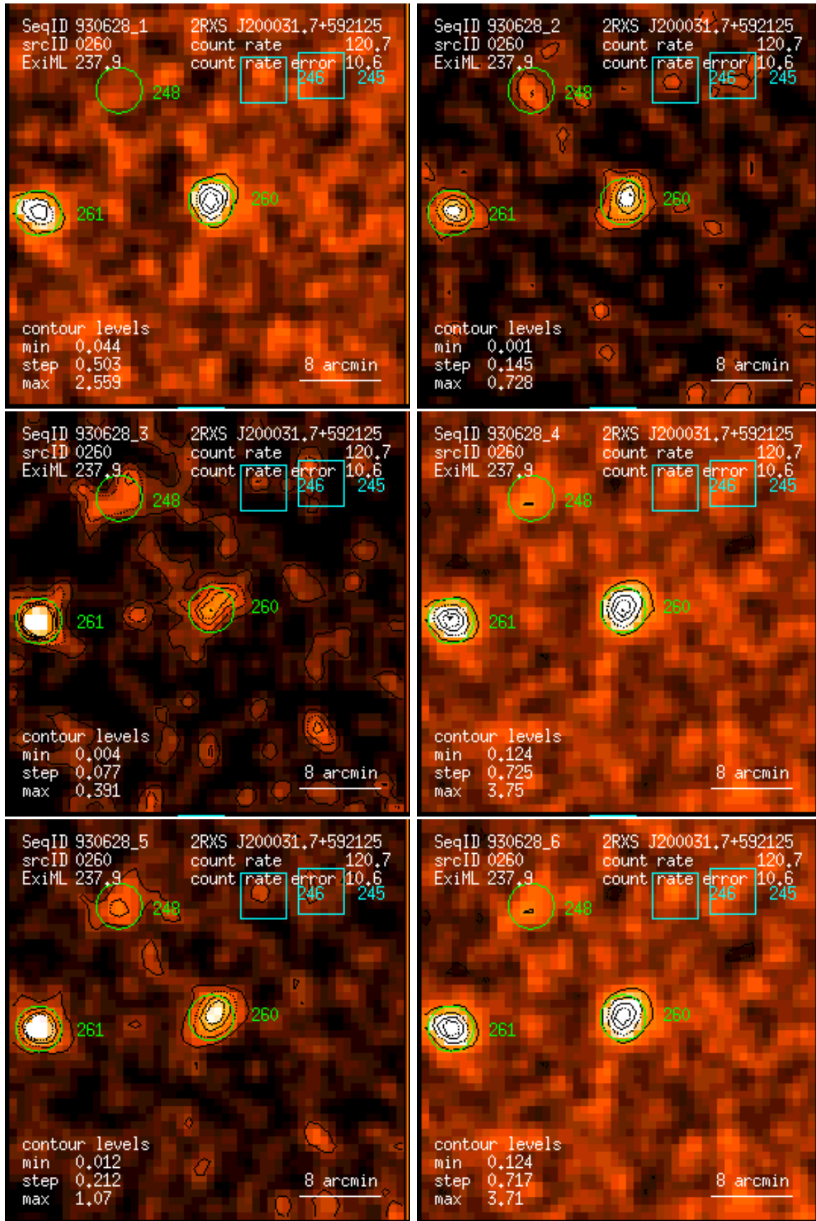
Figure 260: RASS 930628: detection 0260: band rate images, Gaussian filter: (1) PSPC channels 11 – 41, (2) 52 – 90, (3) 91 – 201, (4) 11 – 235, (5) 52 – 201, (6) 11 – 201. Broad band rates in counts/ks. Band rate contour levels in counts/ks/arcmin 2 .
