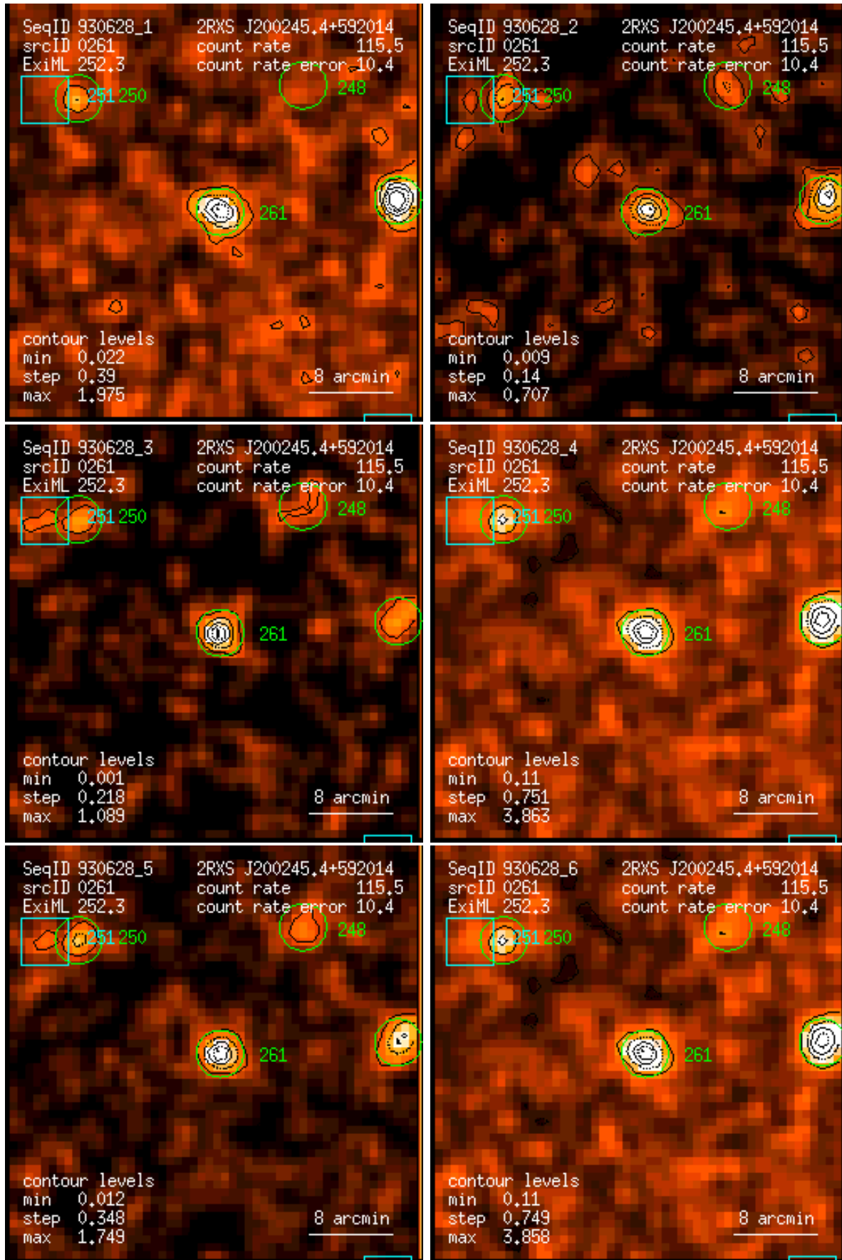
Figure 261: RASS 930628: detection 0261: band rate images, Gaussian filter: (1) PSPC channels 11 – 41, (2) 52 – 90, (3) 91 – 201, (4) 11 – 235, (5) 52 – 201, (6) 11 – 201. Broad band rates in counts/ks. Band rate contour levels in counts/ks/arcmin 2 .
