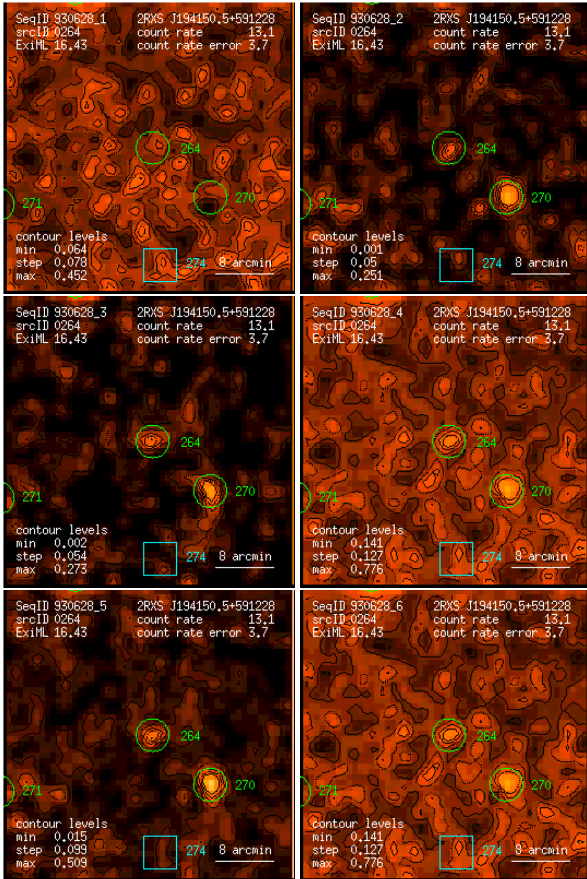
Figure 264: RASS 930628: detection 0264: band rate images, Gaussian filter: (1) PSPC channels 11 – 41, (2) 52 – 90, (3) 91 – 201, (4) 11 – 235, (5) 52 – 201, (6) 11 – 201. Broad band rates in counts/ks. Band rate contour levels in counts/ks/arcmin 2 .
