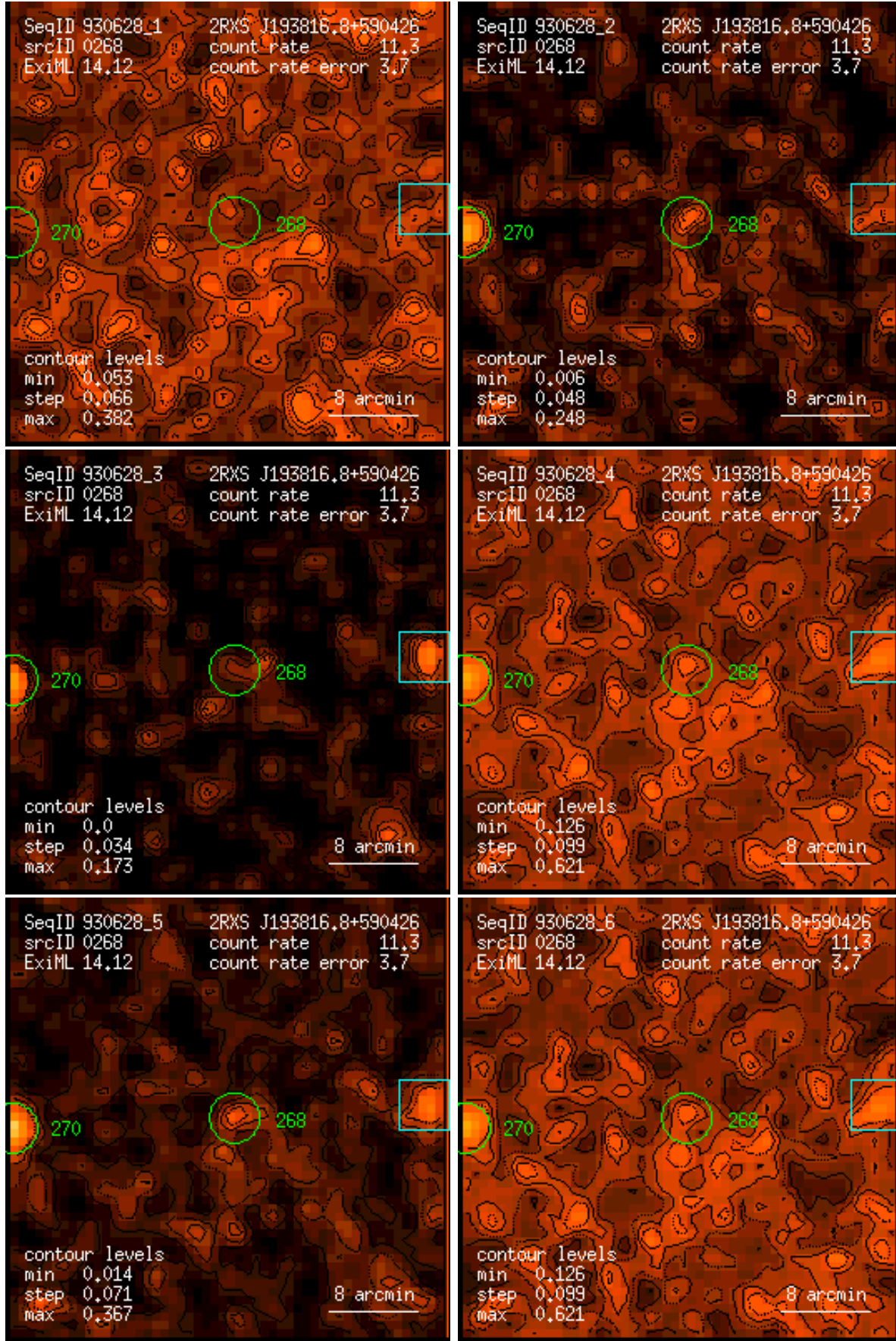
Figure 268: RASS 930628: detection 0268: band rate images, Gaussian filter: (1) PSPC channels 11 – 41, (2) 52 – 90, (3) 91 – 201, (4) 11 – 235, (5) 52 – 201, (6) 11 – 201. Broad band rates in counts/ks. Band rate contour levels in counts/ks/arcmin 2 .
