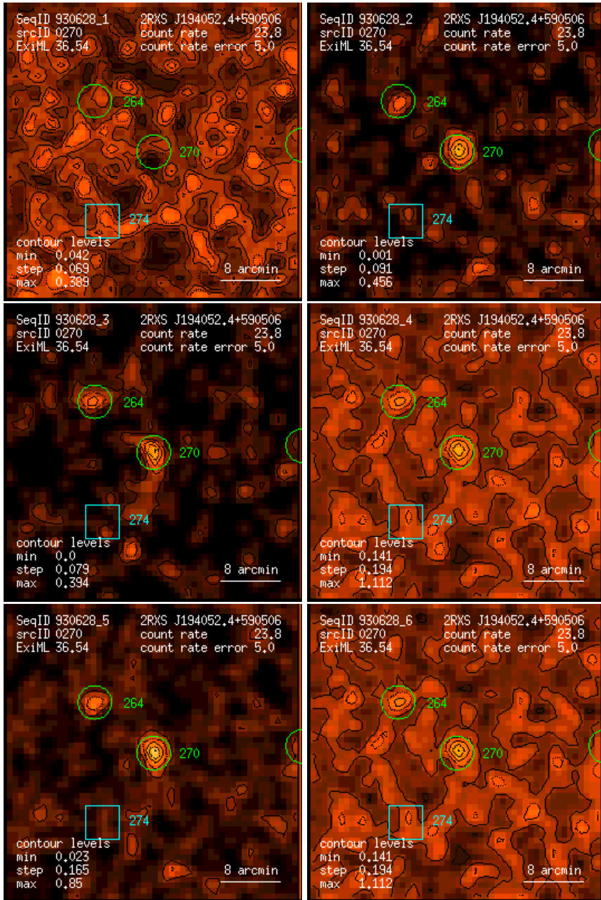
Figure 270: RASS 930628: detection 0270: band rate images, Gaussian filter: (1) PSPC channels 11 – 41, (2) 52 – 90, (3) 91 – 201, (4) 11 – 235, (5) 52 – 201, (6) 11 – 201. Broad band rates in counts/ks. Band rate contour levels in counts/ks/arcmin 2 .
