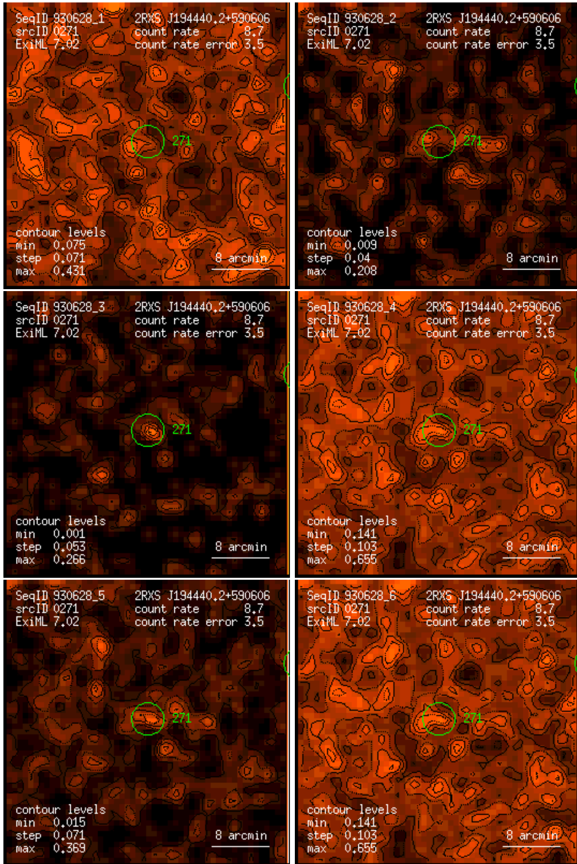
Figure 271: RASS 930628: detection 0271: band rate images, Gaussian filter: (1) PSPC channels 11 – 41, (2) 52 – 90, (3) 91 – 201, (4) 11 – 235, (5) 52 – 201, (6) 11 – 201. Broad band rates in counts/ks. Band rate contour levels in counts/ks/arcmin 2 .
