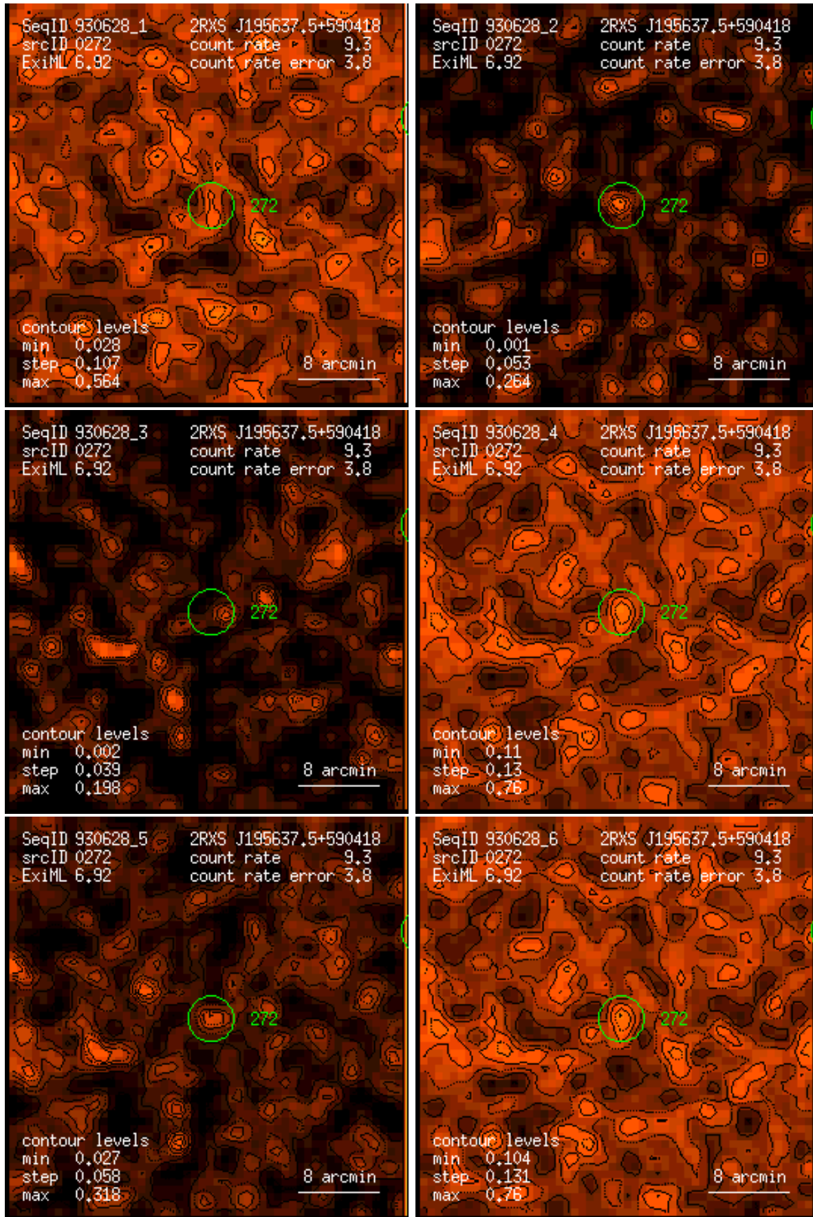
Figure 272: RASS 930628: detection 0272: band rate images, Gaussian filter: (1) PSPC channels 11 – 41, (2) 52 – 90, (3) 91 – 201, (4) 11 – 235, (5) 52 – 201, (6) 11 – 201. Broad band rates in counts/ks. Band rate contour levels in counts/ks/arcmin 2 .
