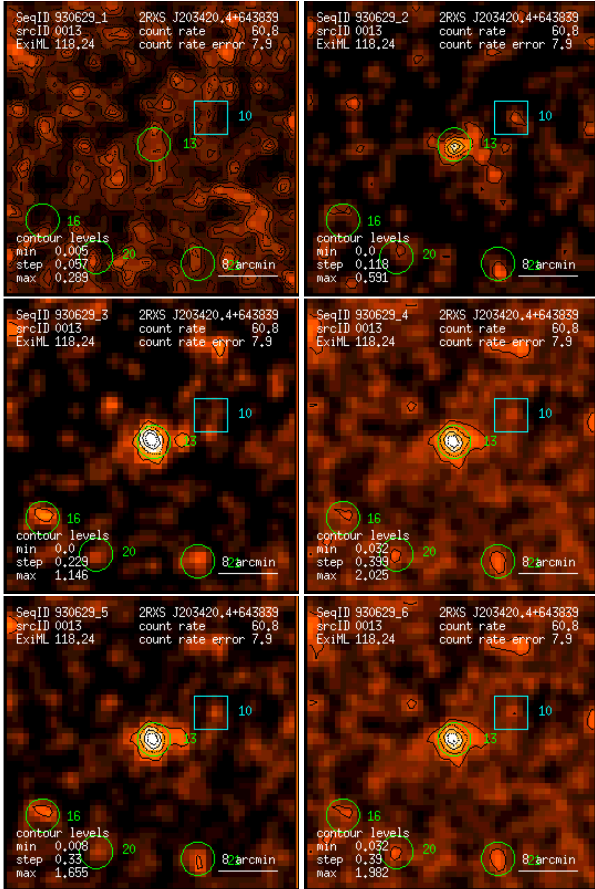
Figure 13: RASS 930629: detection 0013: band rate images, Gaussian filter: (1) PSPC channels 11 – 41, (2) 52 – 90, (3) 91 – 201, (4) 11 – 235, (5) 52 – 201, (6) 11 – 201. Broad band rates in counts/ks. Band rate contour levels in counts/ks/arcmin 2 .
