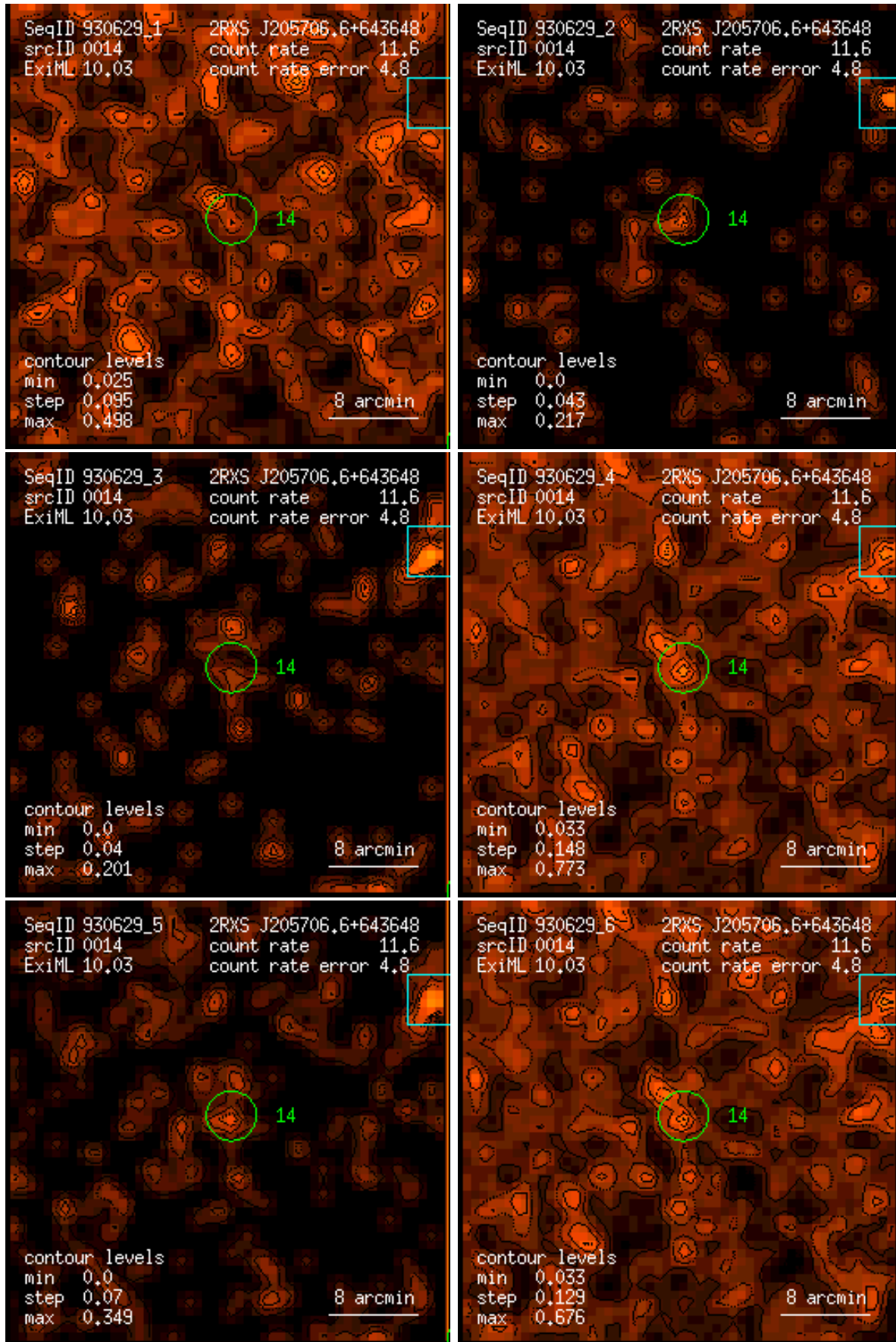
Figure 14: RASS 930629: detection 0014: band rate images, Gaussian filter: (1) PSPC channels 11 – 41, (2) 52 – 90, (3) 91 – 201, (4) 11 – 235, (5) 52 – 201, (6) 11 – 201. Broad band rates in counts/ks. Band rate contour levels in counts/ks/arcmin 2 .
