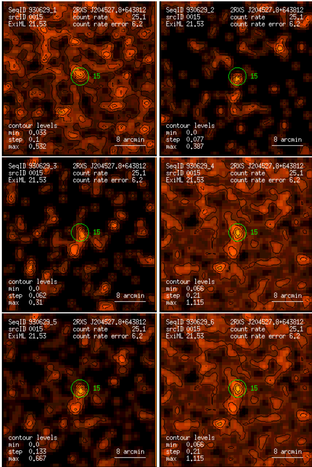
Figure 15: RASS 930629: detection 0015: band rate images, Gaussian filter: (1) PSPC channels 11 – 41, (2) 52 – 90, (3) 91 – 201, (4) 11 – 235, (5) 52 – 201, (6) 11 – 201. Broad band rates in counts/ks. Band rate contour levels in counts/ks/arcmin 2 .
