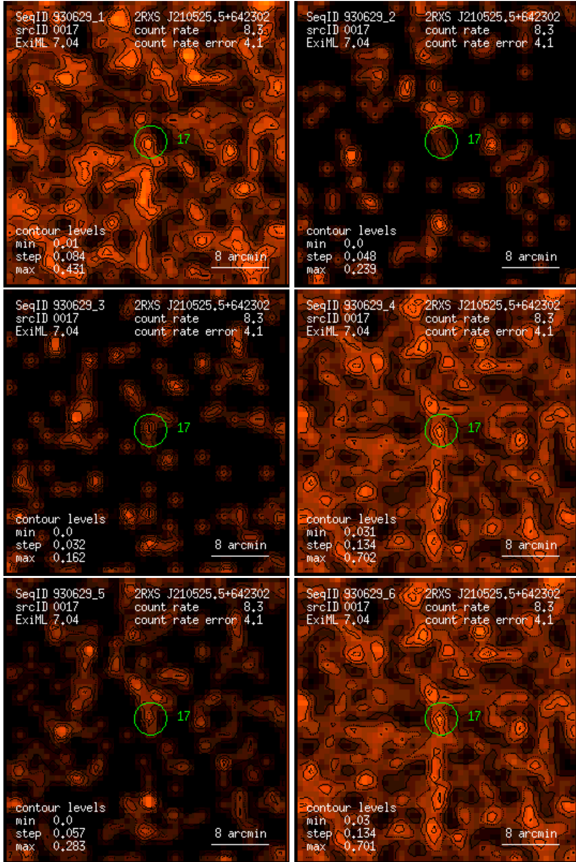
Figure 17: RASS 930629: detection 0017: band rate images, Gaussian filter: (1) PSPC channels 11 – 41, (2) 52 – 90, (3) 91 – 201, (4) 11 – 235, (5) 52 – 201, (6) 11 – 201. Broad band rates in counts/ks. Band rate contour levels in counts/ks/arcmin 2 .
