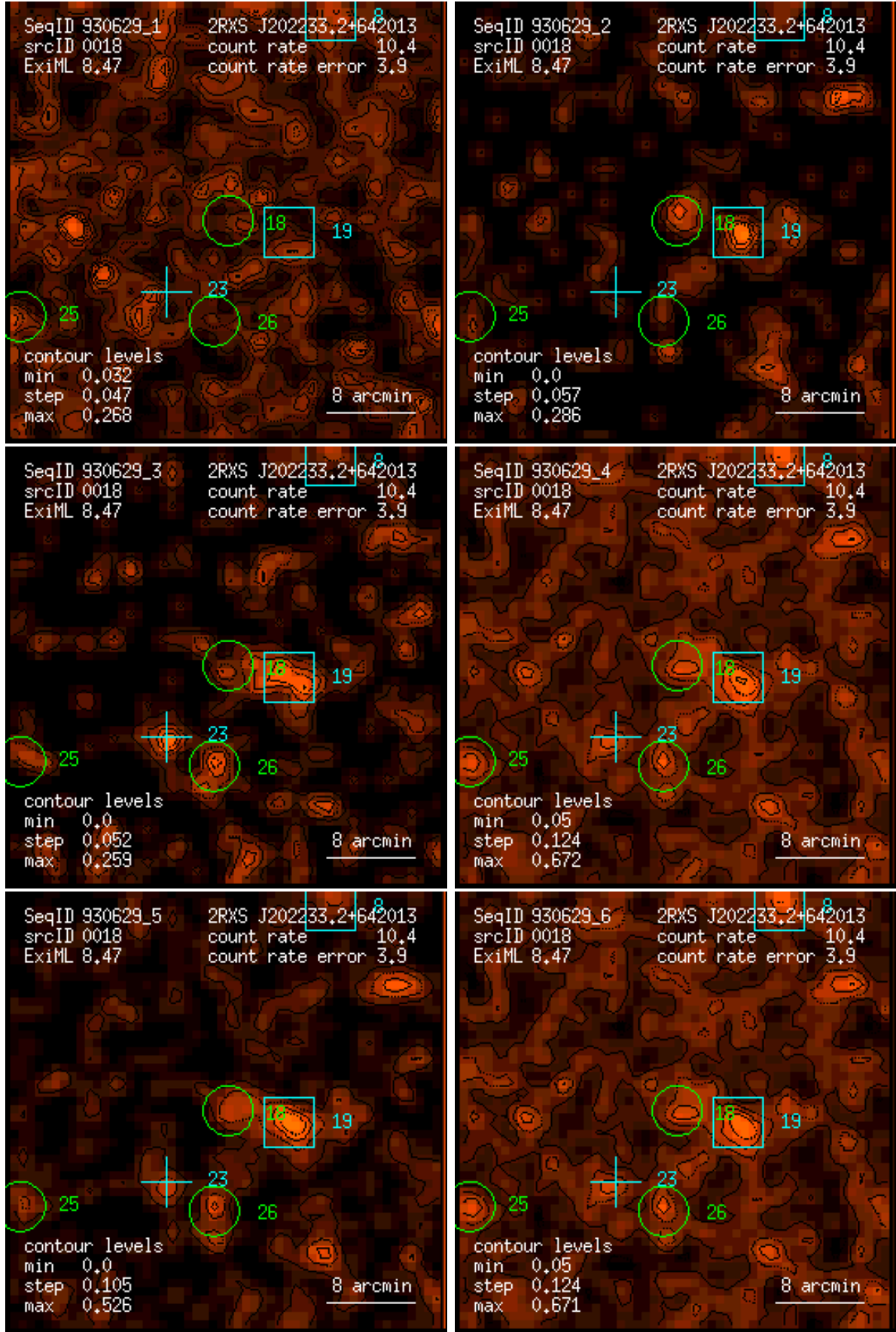
Figure 18: RASS 930629: detection 0018: band rate images, Gaussian filter: (1) PSPC channels 11 – 41, (2) 52 – 90, (3) 91 – 201, (4) 11 – 235, (5) 52 – 201, (6) 11 – 201. Broad band rates in counts/ks. Band rate contour levels in counts/ks/arcmin 2 .
