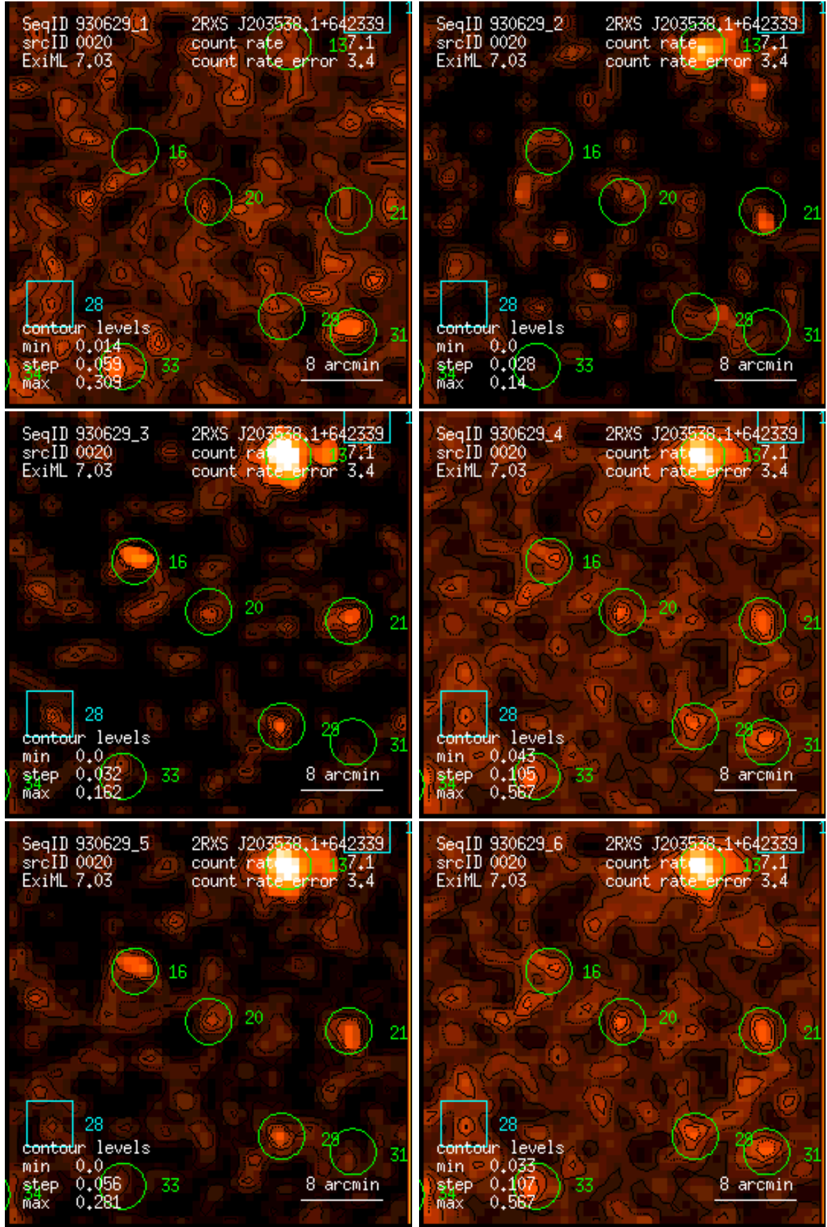
Figure 20: RASS 930629: detection 0020: band rate images, Gaussian filter: (1) PSPC channels 11 – 41, (2) 52 – 90, (3) 91 – 201, (4) 11 – 235, (5) 52 – 201, (6) 11 – 201. Broad band rates in counts/ks. Band rate contour levels in counts/ks/arcmin 2 .
