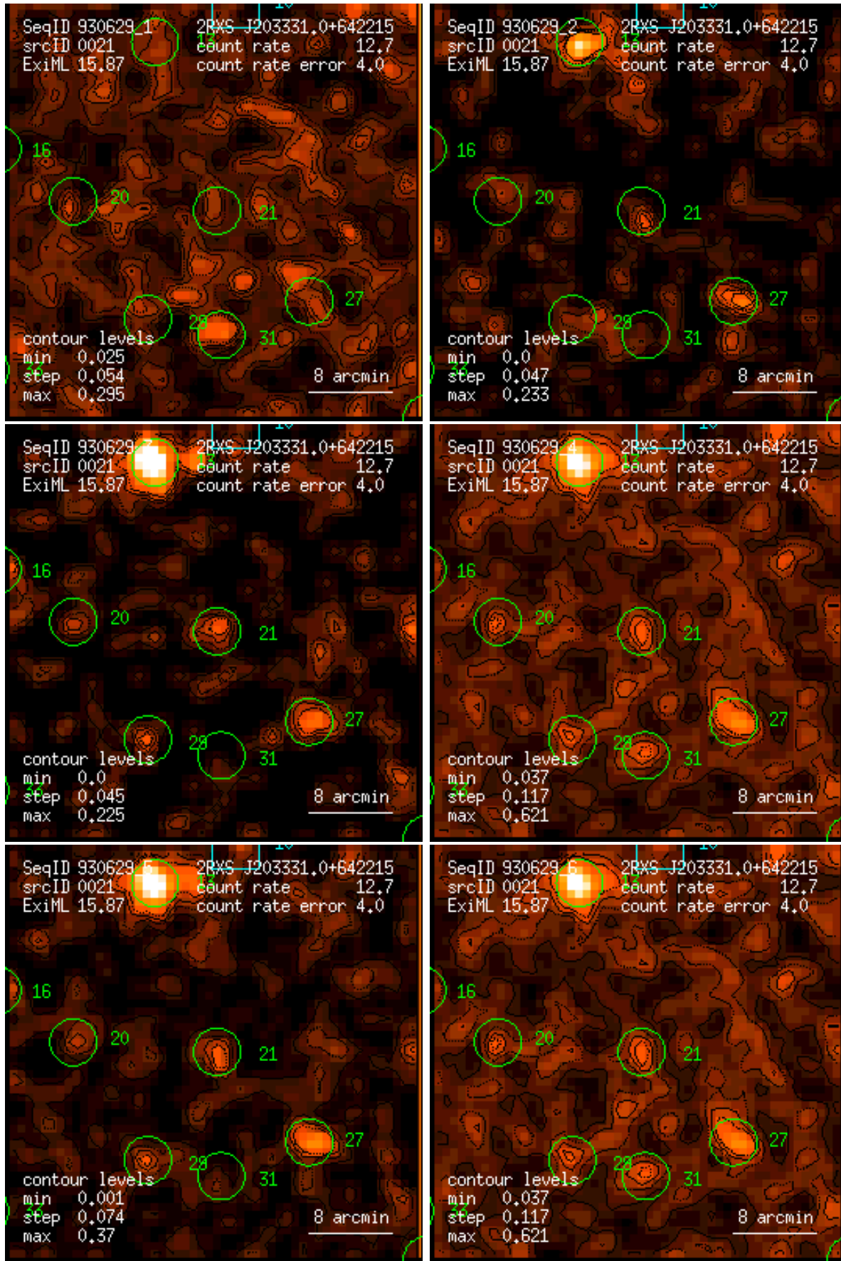
Figure 21: RASS 930629: detection 0021: band rate images, Gaussian filter: (1) PSPC channels 11 – 41, (2) 52 – 90, (3) 91 – 201, (4) 11 – 235, (5) 52 – 201, (6) 11 – 201. Broad band rates in counts/ks. Band rate contour levels in counts/ks/arcmin 2 .
