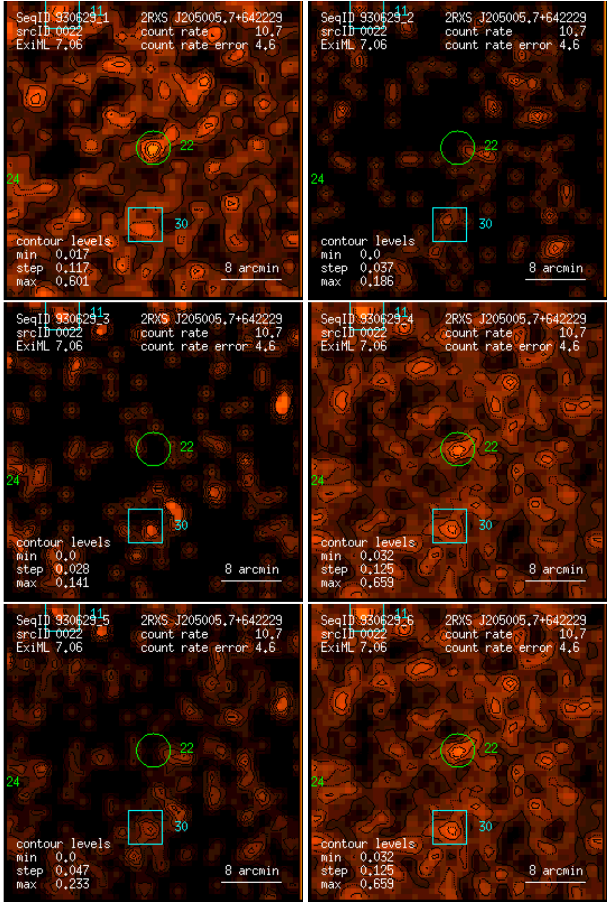
Figure 22: RASS 930629: detection 0022: band rate images, Gaussian filter: (1) PSPC channels 11 – 41, (2) 52 – 90, (3) 91 – 201, (4) 11 – 235, (5) 52 – 201, (6) 11 – 201. Broad band rates in counts/ks. Band rate contour levels in counts/ks/arcmin 2 .
