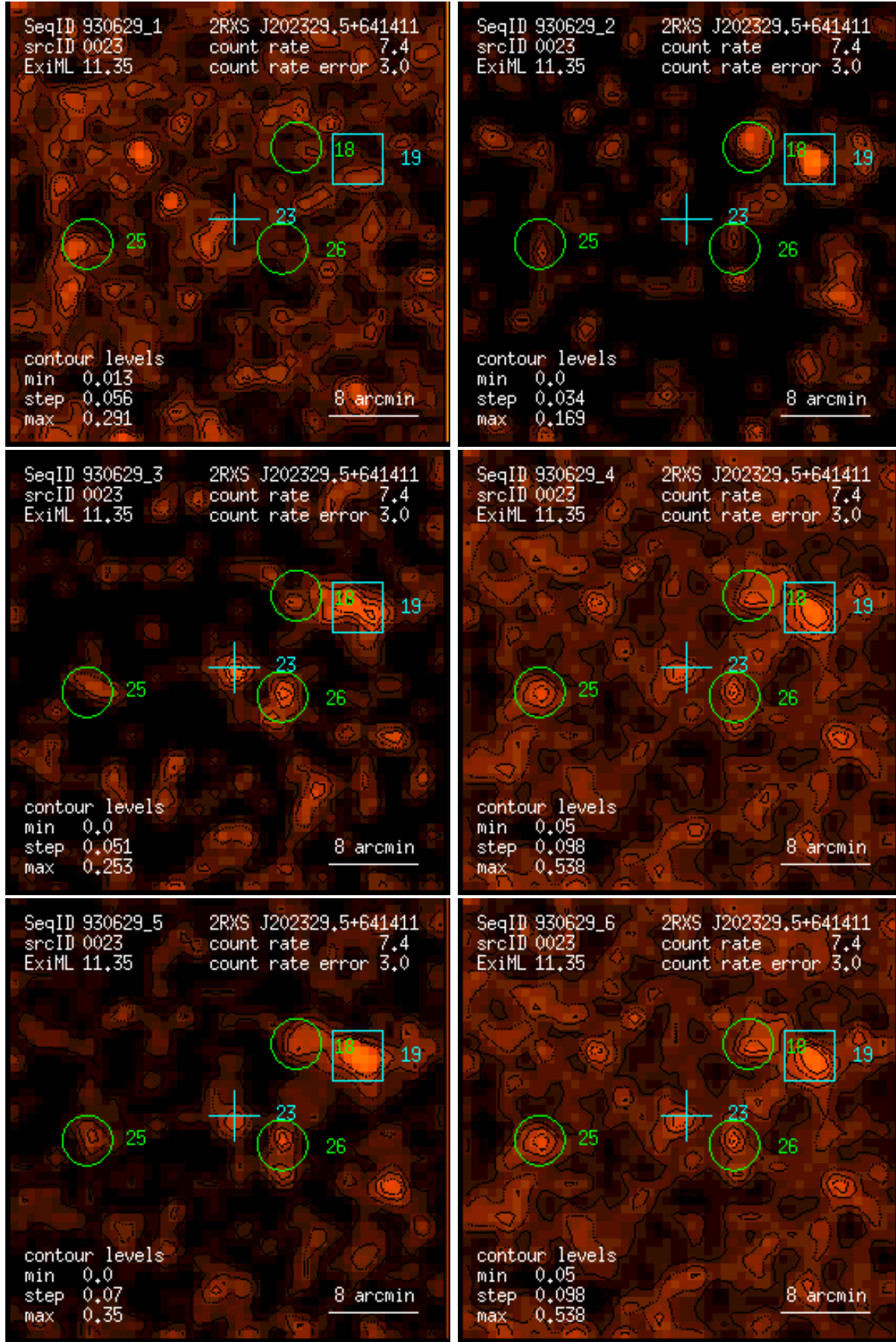
Figure 23: RASS 930629: detection 0023: band rate images, Gaussian filter: (1) PSPC channels 11 – 41, (2) 52 – 90, (3) 91 – 201, (4) 11 – 235, (5) 52 – 201, (6) 11 – 201. Broad band rates in counts/ks. Band rate contour levels in counts/ks/arcmin 2 .
