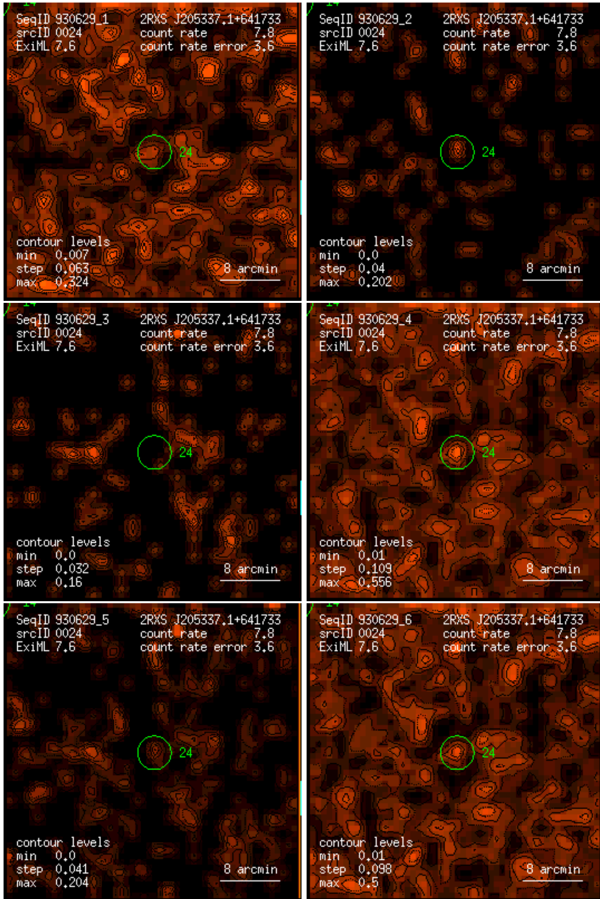
Figure 24: RASS 930629: detection 0024: band rate images, Gaussian filter: (1) PSPC channels 11 – 41, (2) 52 – 90, (3) 91 – 201, (4) 11 – 235, (5) 52 – 201, (6) 11 – 201. Broad band rates in counts/ks. Band rate contour levels in counts/ks/arcmin 2 .
