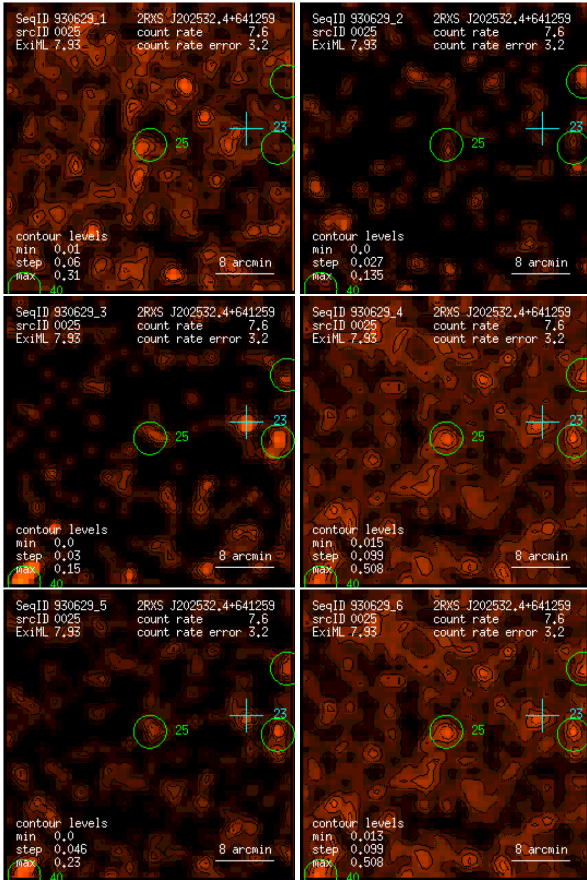
Figure 25: RASS 930629: detection 0025: band rate images, Gaussian filter: (1) PSPC channels 11 – 41, (2) 52 – 90, (3) 91 – 201, (4) 11 – 235, (5) 52 – 201, (6) 11 – 201. Broad band rates in counts/ks. Band rate contour levels in counts/ks/arcmin 2 .
