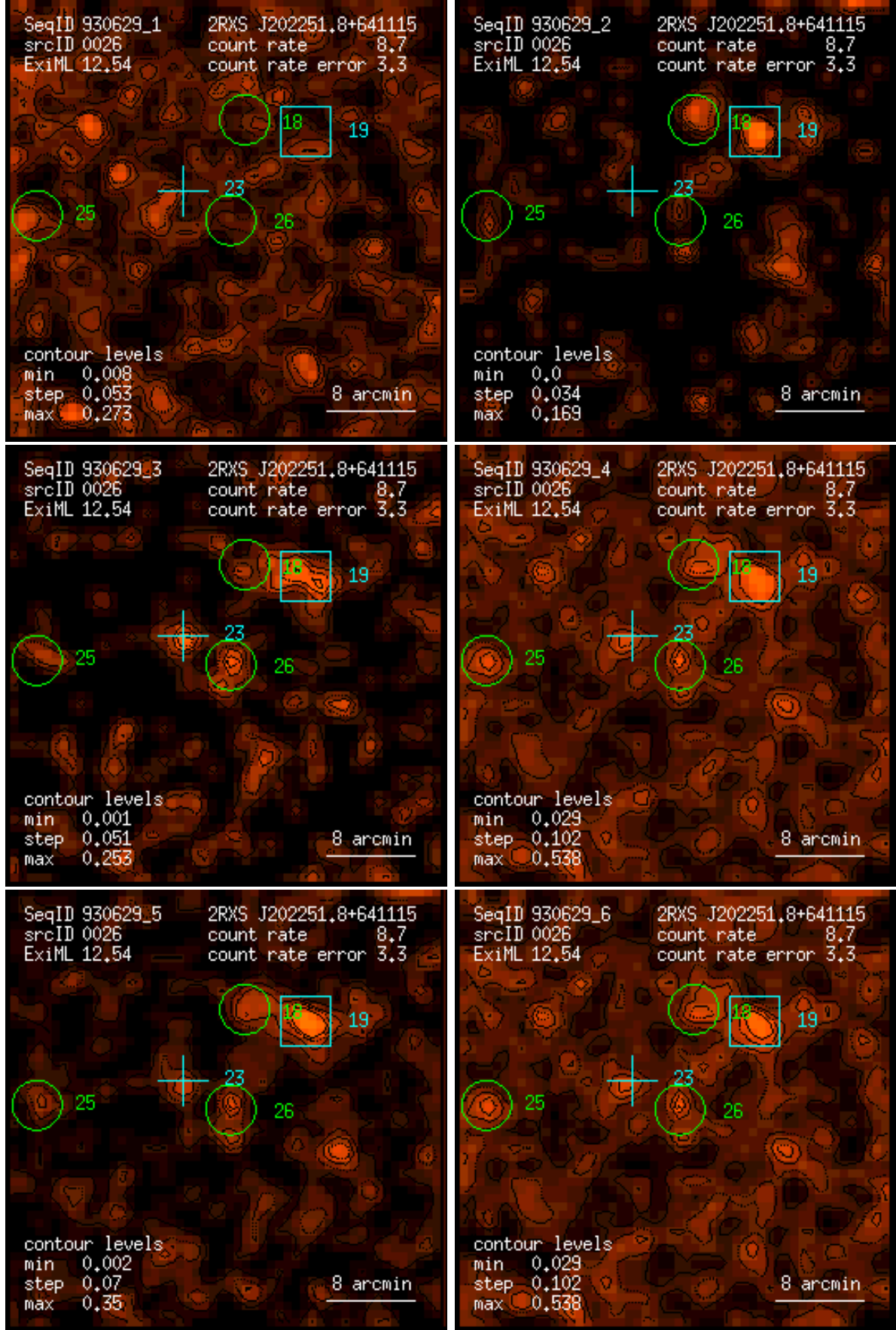
Figure 26: RASS 930629: detection 0026: band rate images, Gaussian filter: (1) PSPC channels 11 – 41, (2) 52 – 90, (3) 91 – 201, (4) 11 – 235, (5) 52 – 201, (6) 11 – 201. Broad band rates in counts/ks. Band rate contour levels in counts/ks/arcmin 2 .
