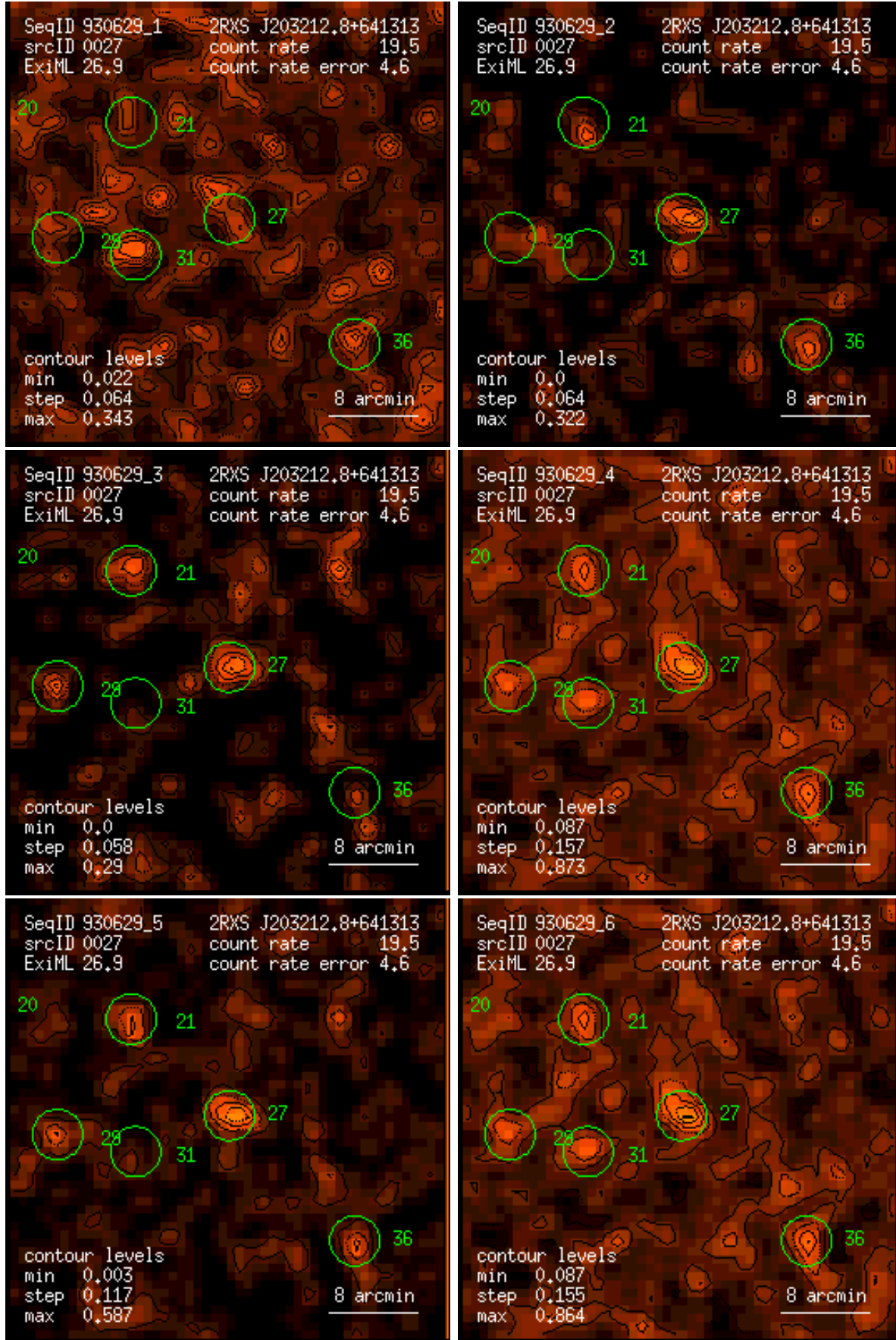
Figure 27: RASS 930629: detection 0027: band rate images, Gaussian filter: (1) PSPC channels 11 – 41, (2) 52 – 90, (3) 91 – 201, (4) 11 – 235, (5) 52 – 201, (6) 11 – 201. Broad band rates in counts/ks. Band rate contour levels in counts/ks/arcmin 2 .
