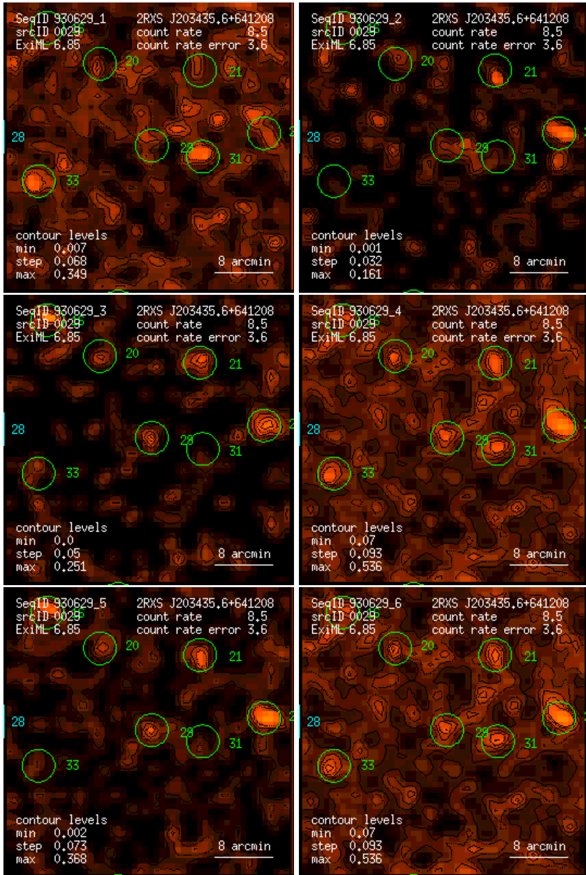
Figure 29: RASS 930629: detection 0029: band rate images, Gaussian filter: (1) PSPC channels 11 – 41, (2) 52 – 90, (3) 91 – 201, (4) 11 – 235, (5) 52 – 201, (6) 11 – 201. Broad band rates in counts/ks. Band rate contour levels in counts/ks/arcmin 2 .
