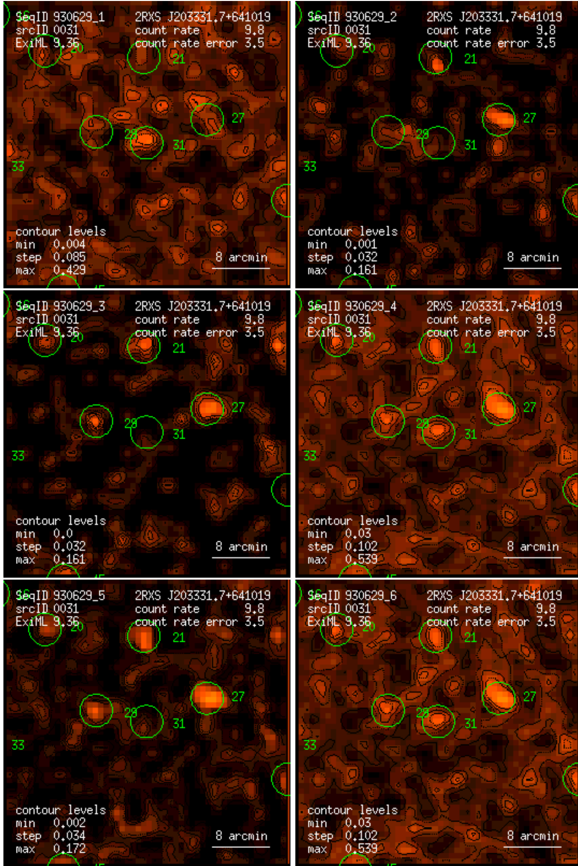
Figure 31: RASS 930629: detection 0031: band rate images, Gaussian filter: (1) PSPC channels 11 – 41, (2) 52 – 90, (3) 91 – 201, (4) 11 – 235, (5) 52 – 201, (6) 11 – 201. Broad band rates in counts/ks. Band rate contour levels in counts/ks/arcmin 2 .
