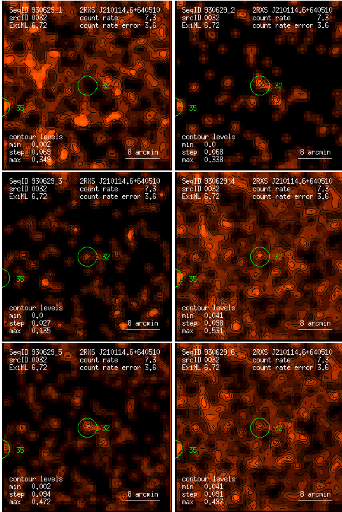
Figure 32: RASS 930629: detection 0032: band rate images, Gaussian filter: (1) PSPC channels 11 – 41, (2) 52 – 90, (3) 91 – 201, (4) 11 – 235, (5) 52 – 201, (6) 11 – 201. Broad band rates in counts/ks. Band rate contour levels in counts/ks/arcmin 2 .
