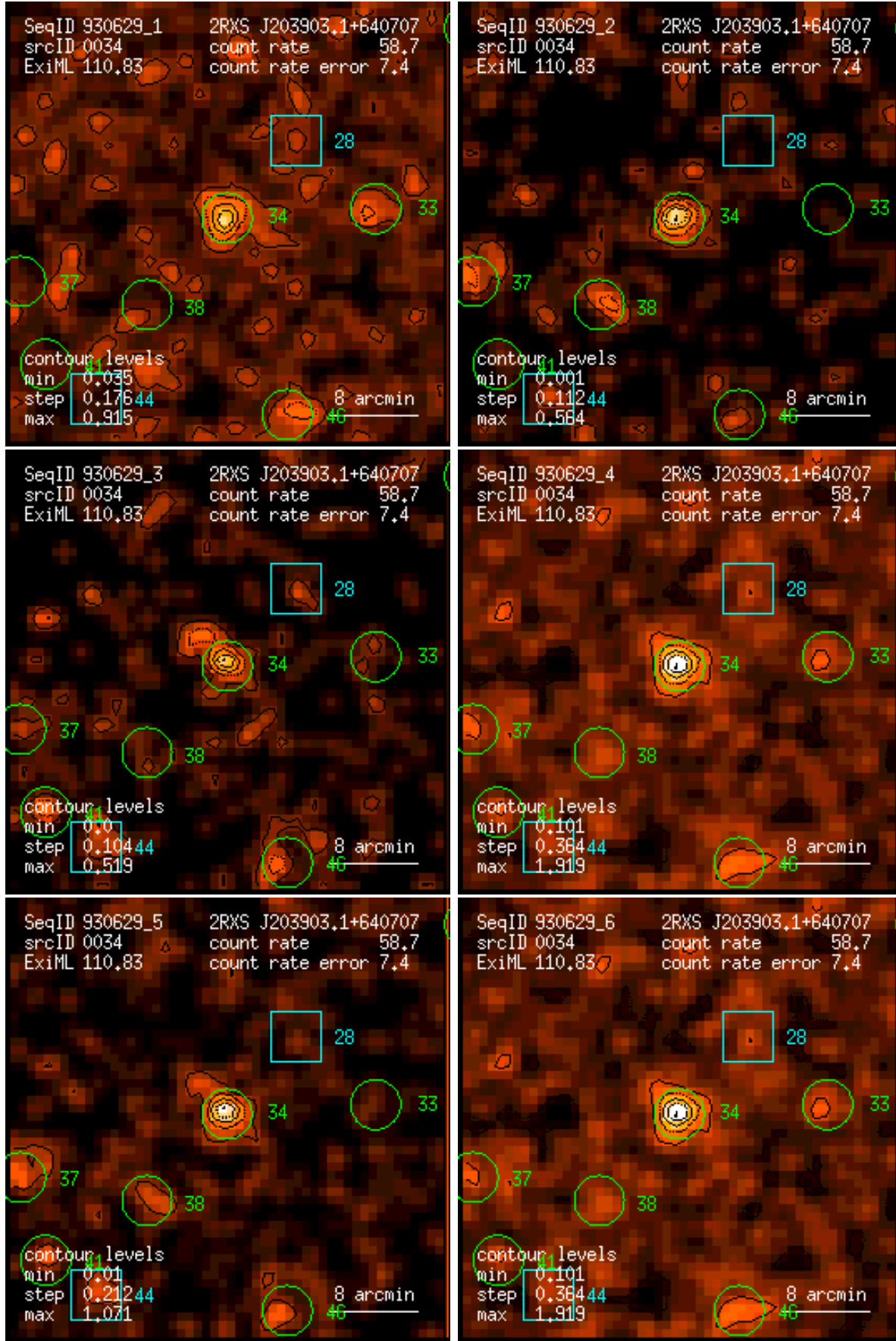
Figure 34: RASS 930629: detection 0034: band rate images, Gaussian filter: (1) PSPC channels 11 – 41, (2) 52 – 90, (3) 91 – 201, (4) 11 – 235, (5) 52 – 201, (6) 11 – 201. Broad band rates in counts/ks. Band rate contour levels in counts/ks/arcmin 2 .
