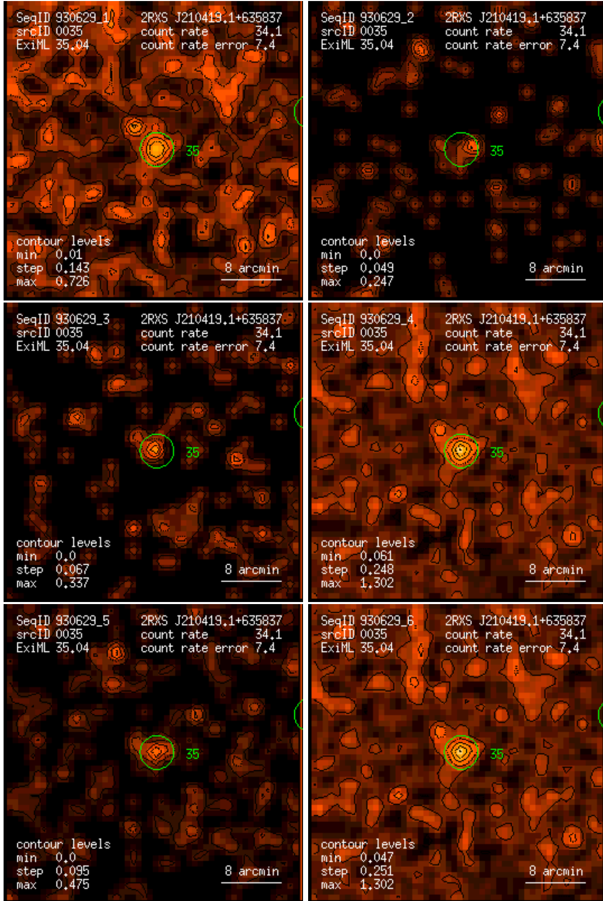
Figure 35: RASS 930629: detection 0035: band rate images, Gaussian filter: (1) PSPC channels 11 – 41, (2) 52 – 90, (3) 91 – 201, (4) 11 – 235, (5) 52 – 201, (6) 11 – 201. Broad band rates in counts/ks. Band rate contour levels in counts/ks/arcmin 2 .
