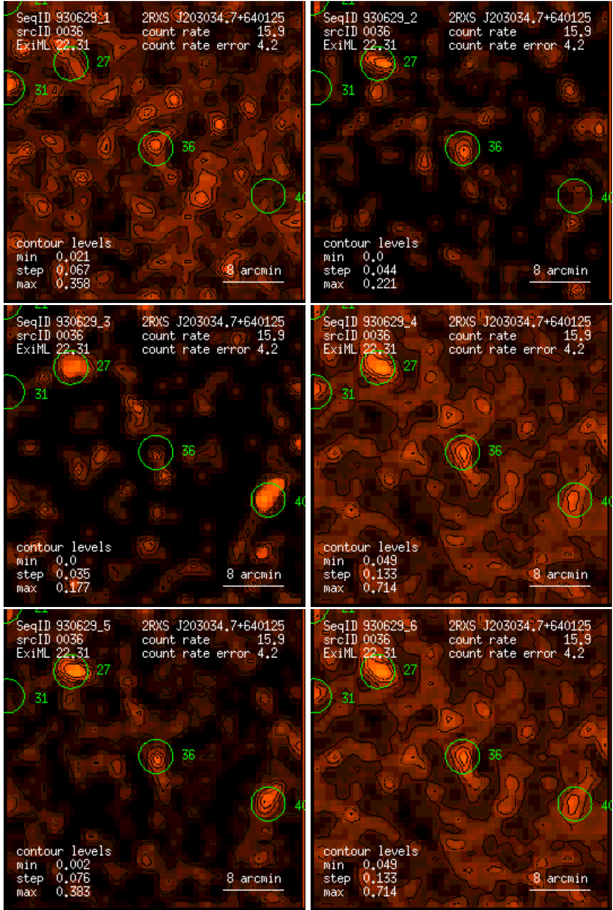
Figure 36: RASS 930629: detection 0036: band rate images, Gaussian filter: (1) PSPC channels 11 – 41, (2) 52 – 90, (3) 91 – 201, (4) 11 – 235, (5) 52 – 201, (6) 11 – 201. Broad band rates in counts/ks. Band rate contour levels in counts/ks/arcmin 2 .
