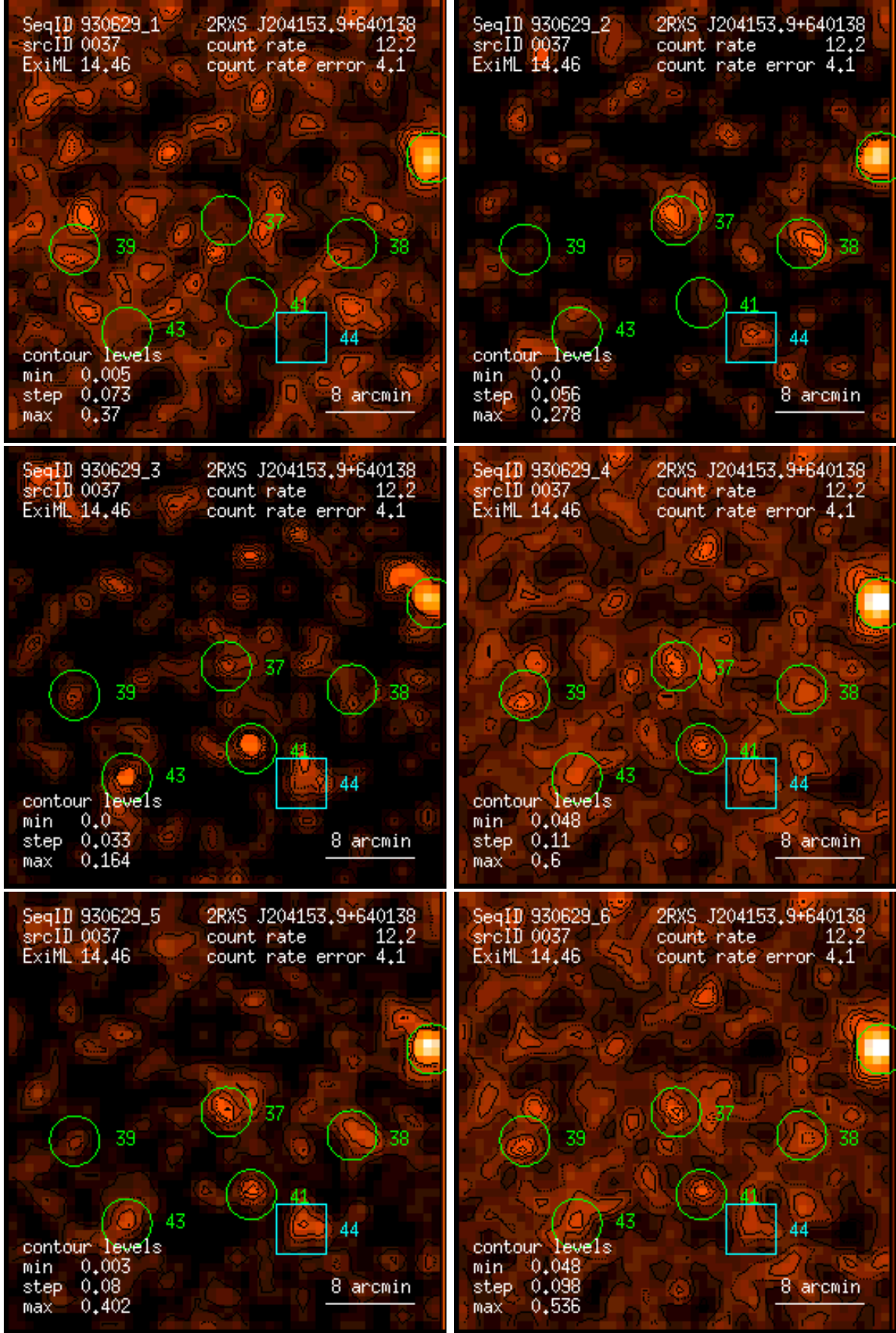
Figure 37: RASS 930629: detection 0037: band rate images, Gaussian filter: (1) PSPC channels 11 – 41, (2) 52 – 90, (3) 91 – 201, (4) 11 – 235, (5) 52 – 201, (6) 11 – 201. Broad band rates in counts/ks. Band rate contour levels in counts/ks/arcmin 2 .
