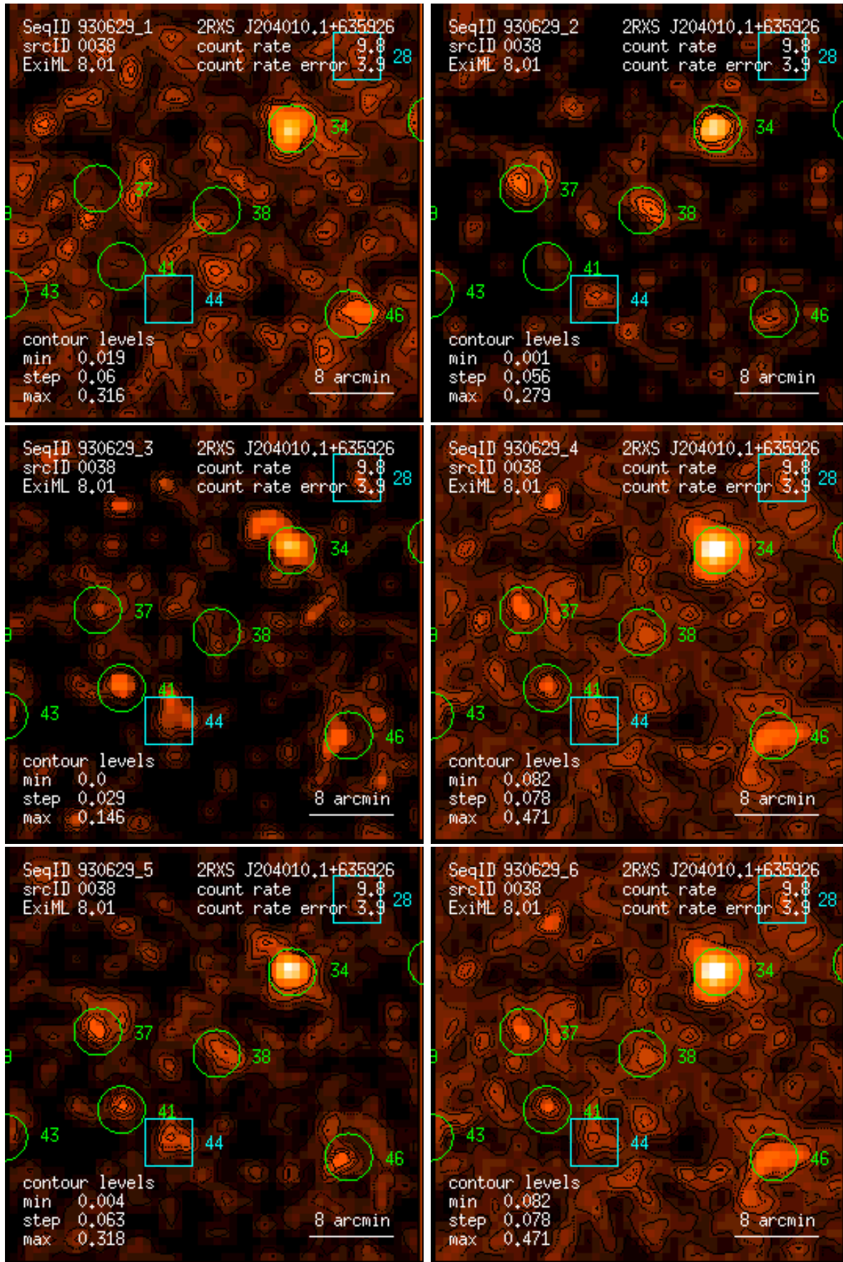
Figure 38: RASS 930629: detection 0038: band rate images, Gaussian filter: (1) PSPC channels 11 – 41, (2) 52 – 90, (3) 91 – 201, (4) 11 – 235, (5) 52 – 201, (6) 11 – 201. Broad band rates in counts/ks. Band rate contour levels in counts/ks/arcmin 2 .
