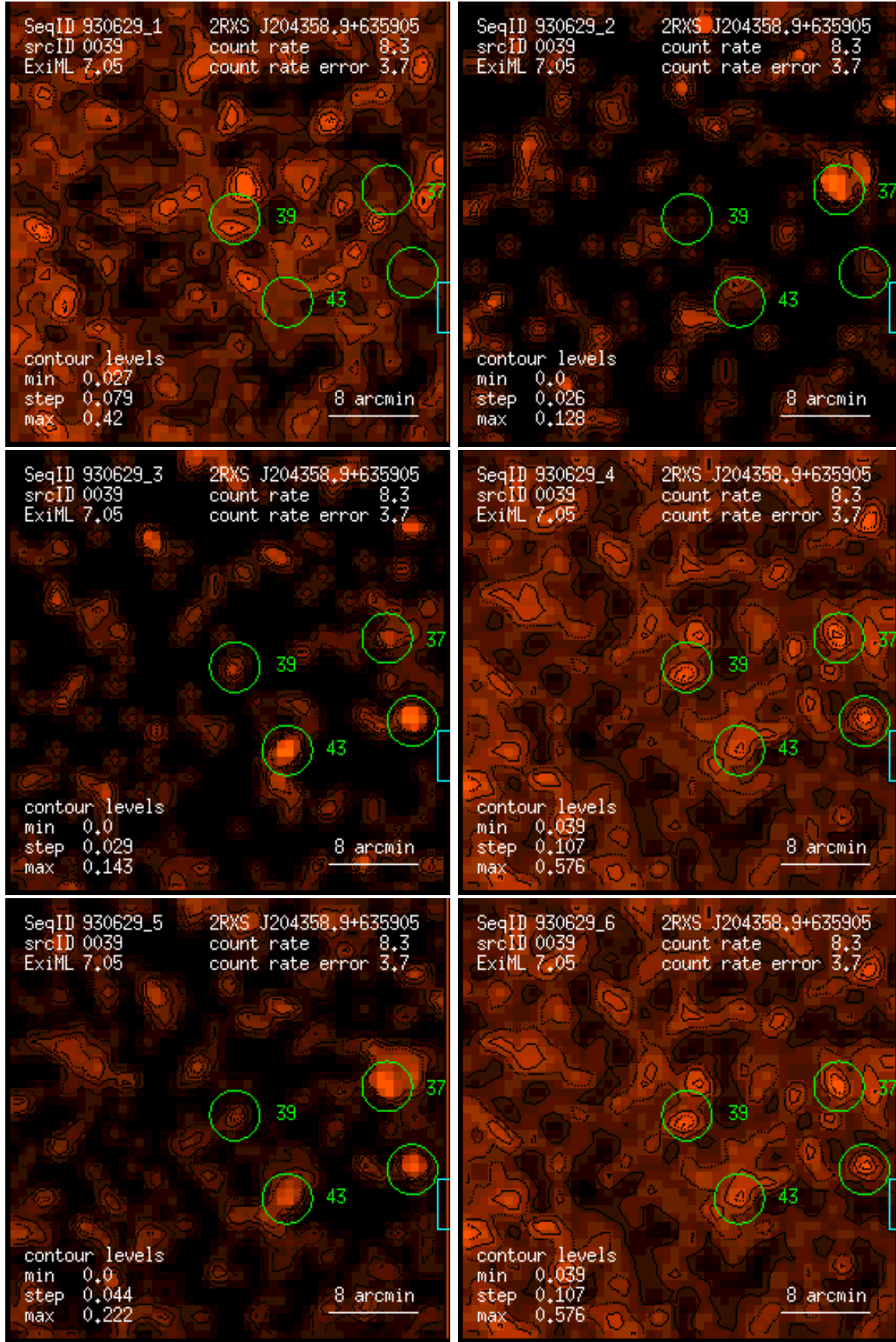
Figure 39: RASS 930629: detection 0039: band rate images, Gaussian filter: (1) PSPC channels 11 – 41, (2) 52 – 90, (3) 91 – 201, (4) 11 – 235, (5) 52 – 201, (6) 11 – 201. Broad band rates in counts/ks. Band rate contour levels in counts/ks/arcmin 2 .
