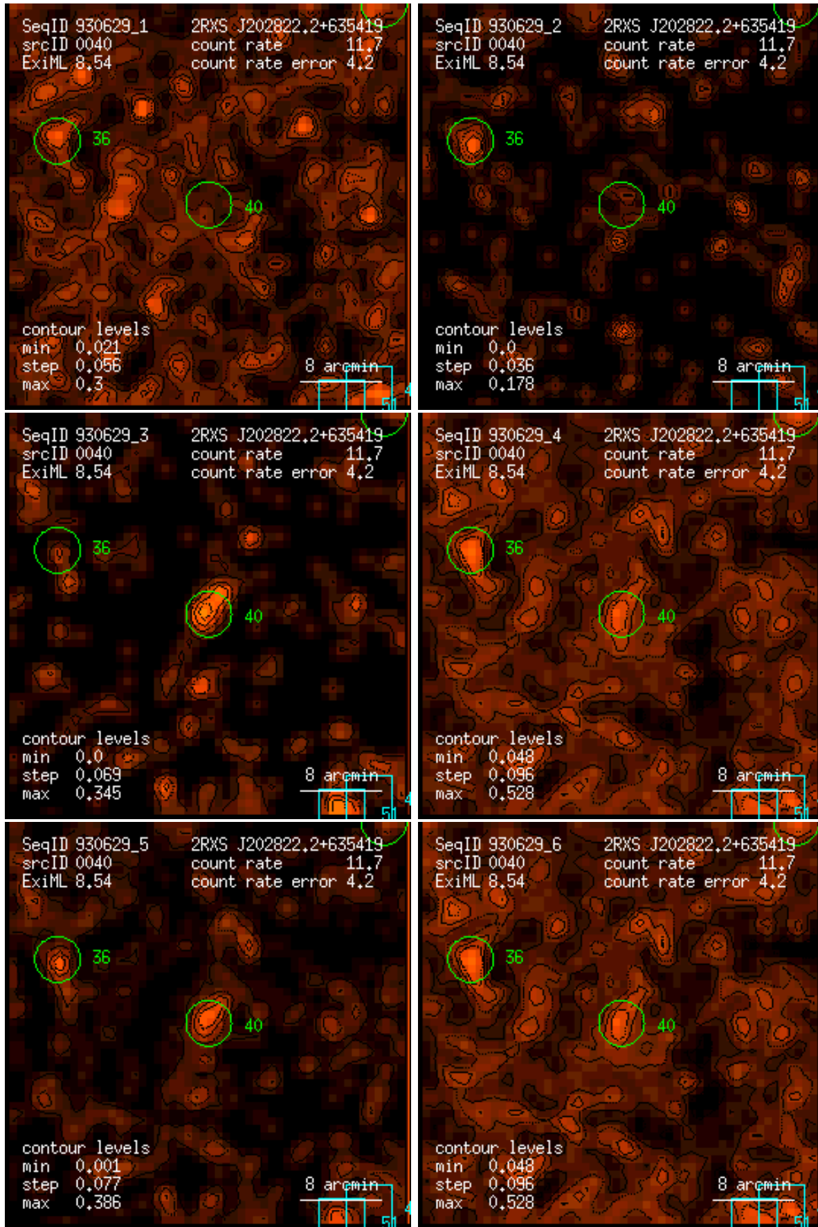
Figure 40: RASS 930629: detection 0040: band rate images, Gaussian filter: (1) PSPC channels 11 – 41, (2) 52 – 90, (3) 91 – 201, (4) 11 – 235, (5) 52 – 201, (6) 11 – 201. Broad band rates in counts/ks. Band rate contour levels in counts/ks/arcmin 2 .
