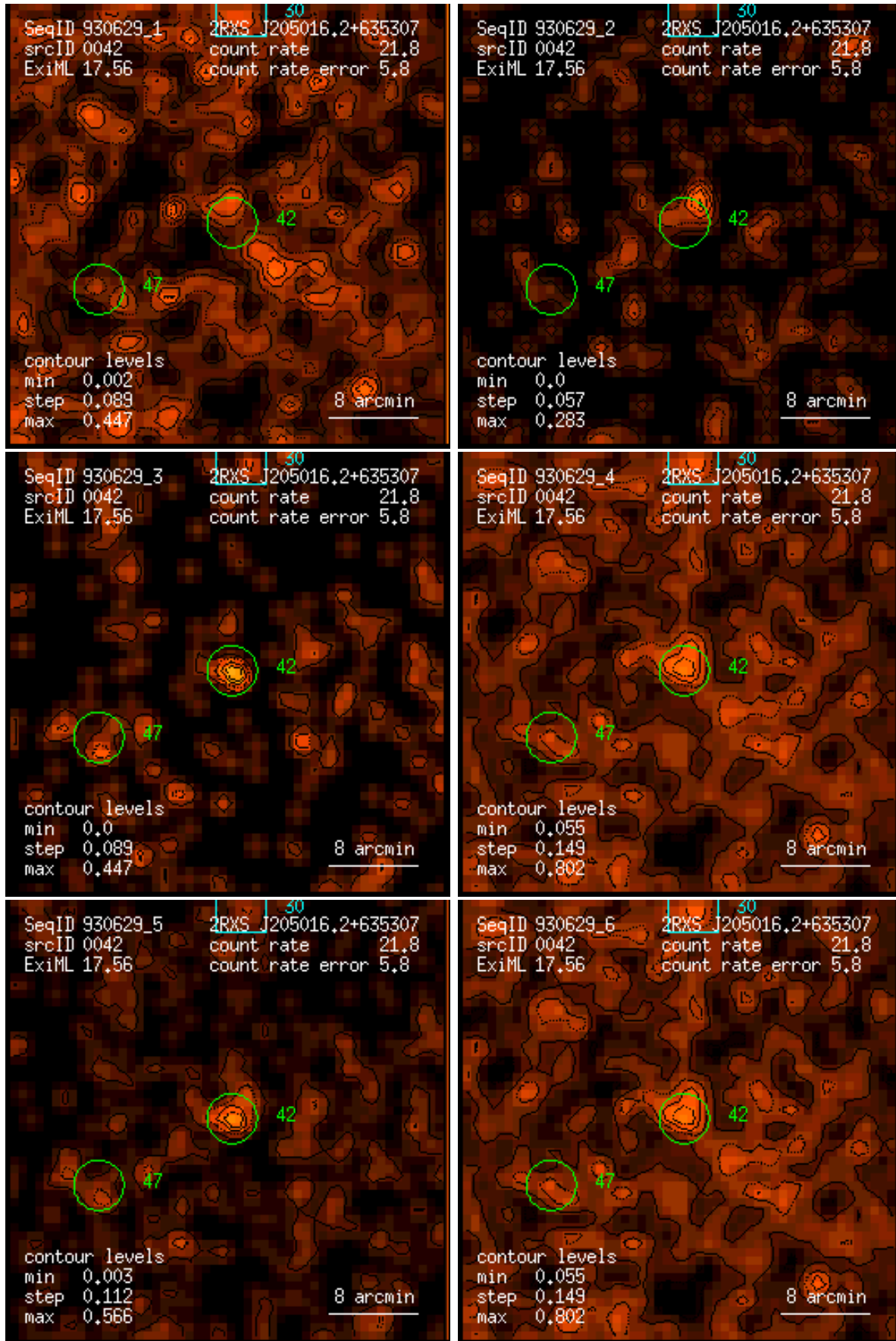
Figure 42: RASS 930629: detection 0042: band rate images, Gaussian filter: (1) PSPC channels 11 – 41, (2) 52 – 90, (3) 91 – 201, (4) 11 – 235, (5) 52 – 201, (6) 11 – 201. Broad band rates in counts/ks. Band rate contour levels in counts/ks/arcmin 2 .
