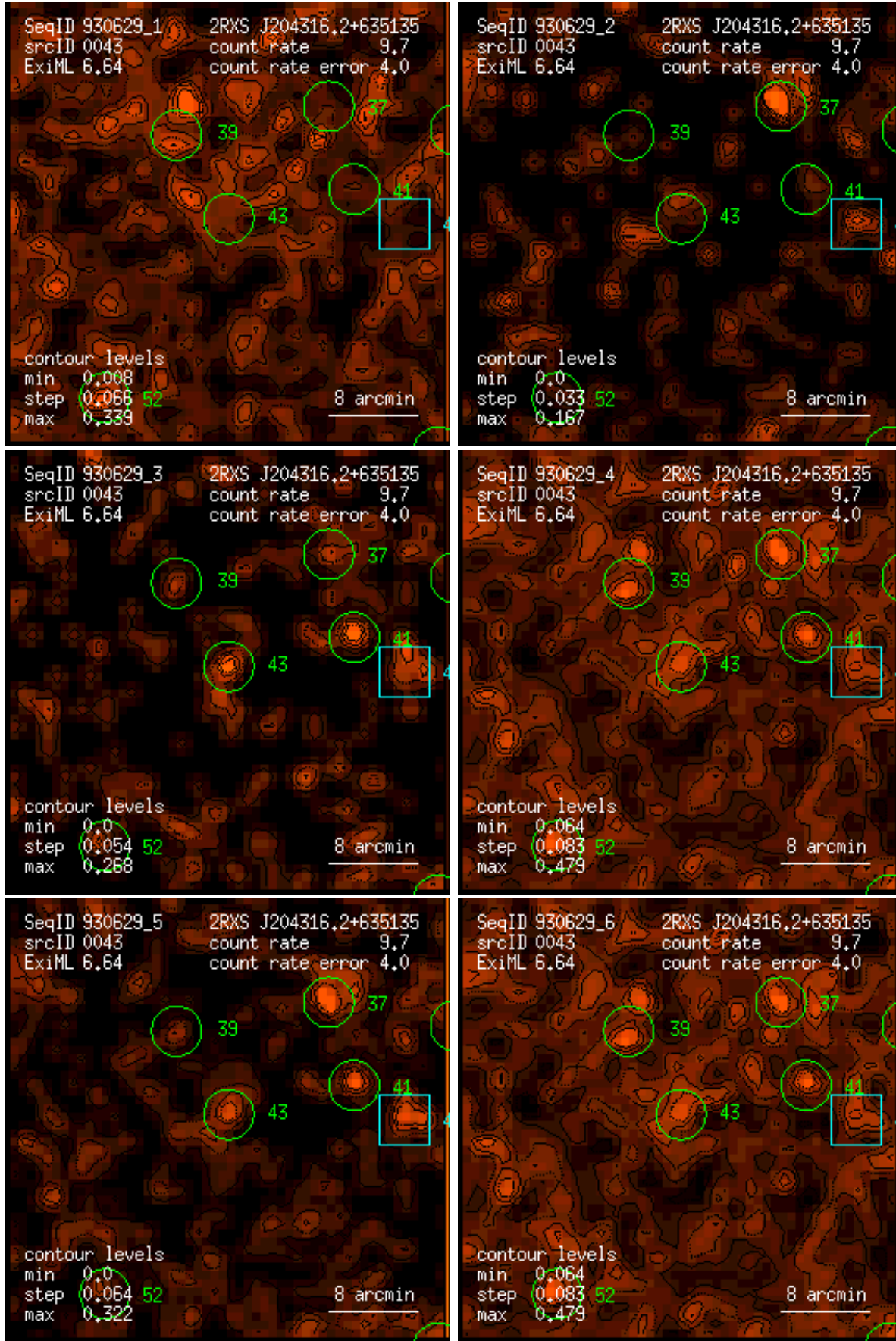
Figure 43: RASS 930629: detection 0043: band rate images, Gaussian filter: (1) PSPC channels 11 – 41, (2) 52 – 90, (3) 91 – 201, (4) 11 – 235, (5) 52 – 201, (6) 11 – 201. Broad band rates in counts/ks. Band rate contour levels in counts/ks/arcmin 2 .
