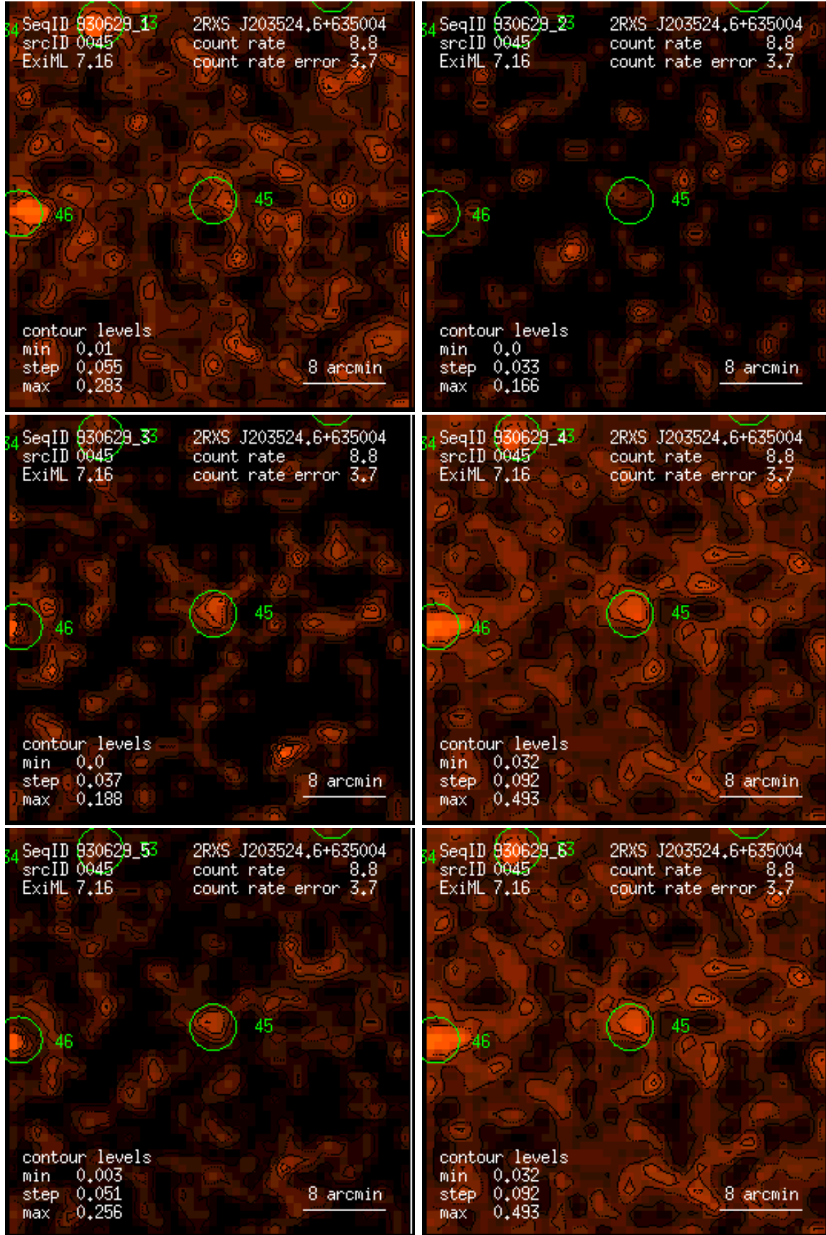
Figure 45: RASS 930629: detection 0045: band rate images, Gaussian filter: (1) PSPC channels 11 – 41, (2) 52 – 90, (3) 91 – 201, (4) 11 – 235, (5) 52 – 201, (6) 11 – 201. Broad band rates in counts/ks. Band rate contour levels in counts/ks/arcmin 2 .
