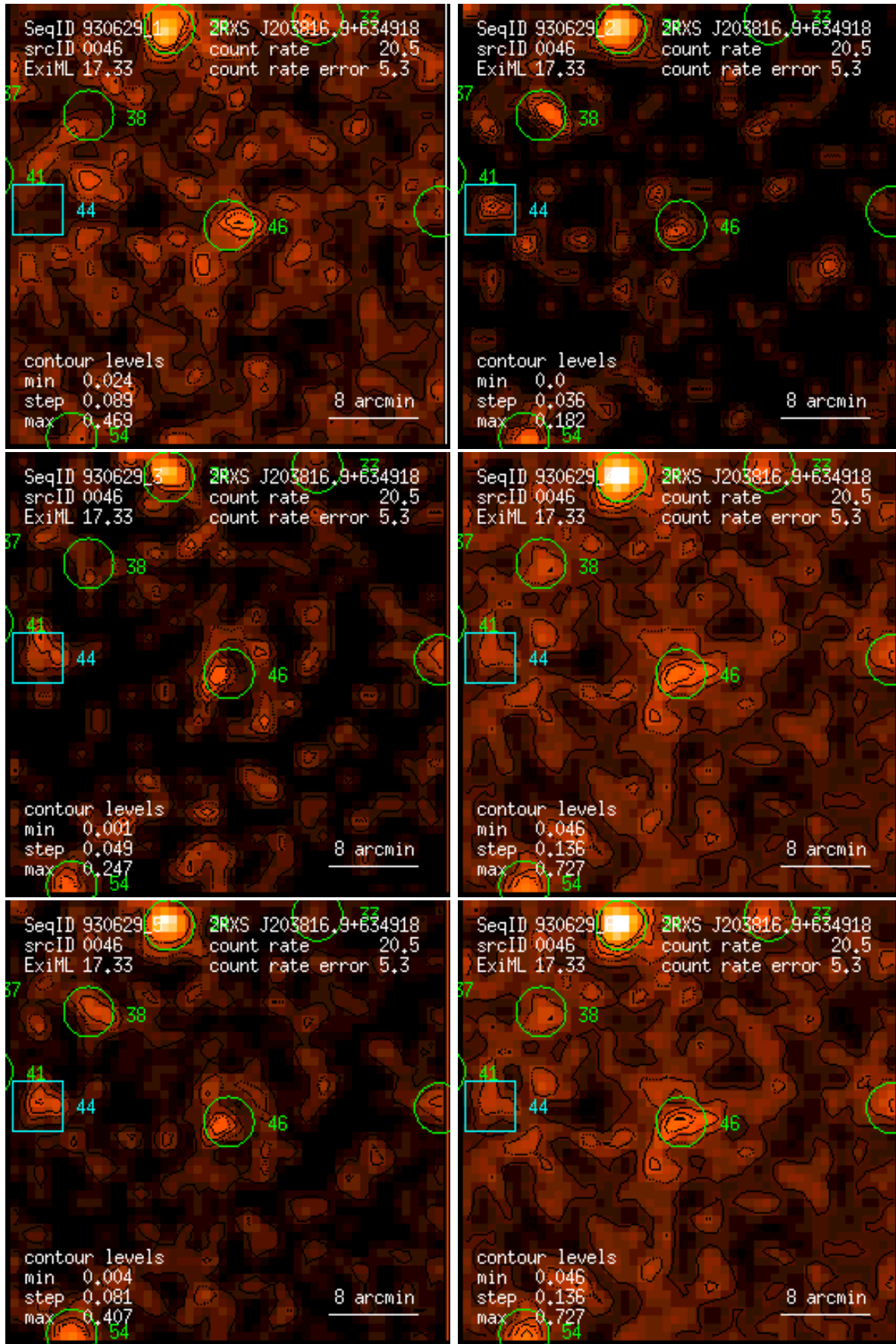
Figure 46: RASS 930629: detection 0046: band rate images, Gaussian filter: (1) PSPC channels 11 – 41, (2) 52 – 90, (3) 91 – 201, (4) 11 – 235, (5) 52 – 201, (6) 11 – 201. Broad band rates in counts/ks. Band rate contour levels in counts/ks/arcmin 2 .
