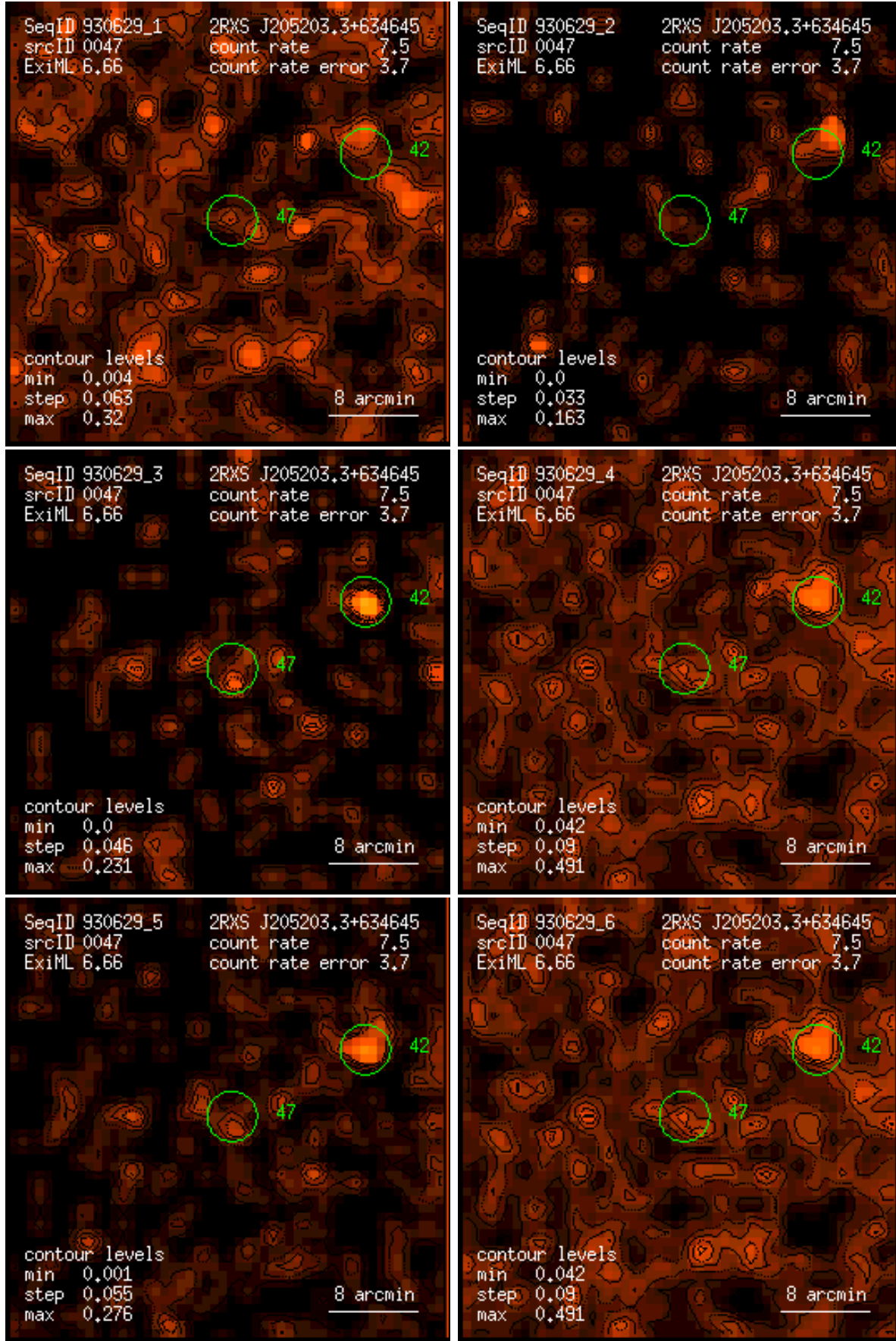
Figure 47: RASS 930629: detection 0047: band rate images, Gaussian filter: (1) PSPC channels 11 – 41, (2) 52 – 90, (3) 91 – 201, (4) 11 – 235, (5) 52 – 201, (6) 11 – 201. Broad band rates in counts/ks. Band rate contour levels in counts/ks/arcmin 2 .
