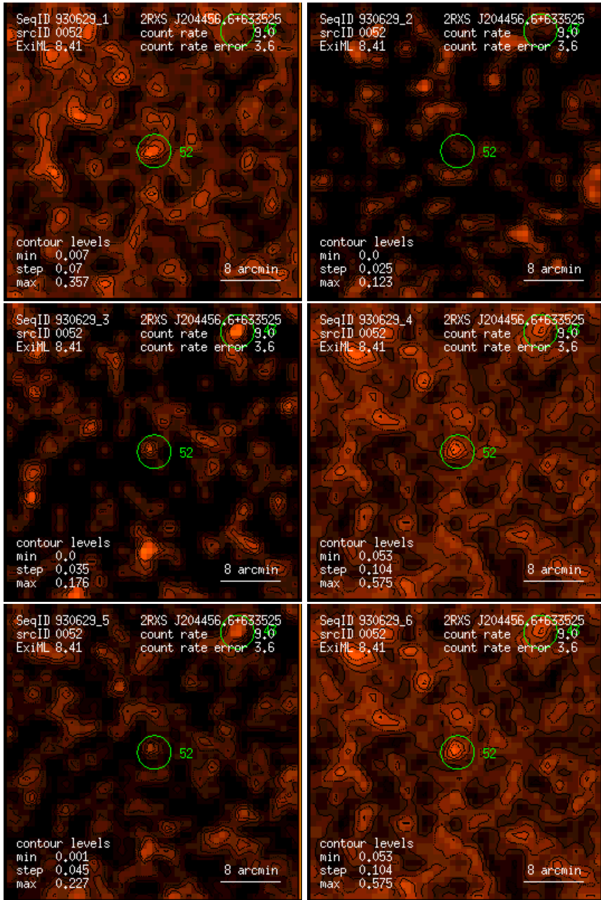
Figure 52: RASS 930629: detection 0052: band rate images, Gaussian filter: (1) PSPC channels 11 – 41, (2) 52 – 90, (3) 91 – 201, (4) 11 – 235, (5) 52 – 201, (6) 11 – 201. Broad band rates in counts/ks. Band rate contour levels in counts/ks/arcmin 2 .
