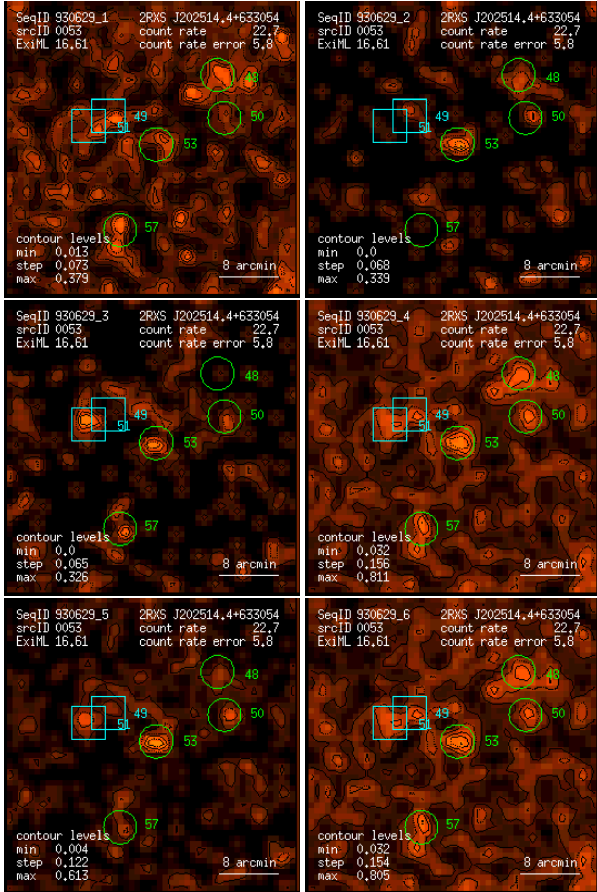
Figure 53: RASS 930629: detection 0053: band rate images, Gaussian filter: (1) PSPC channels 11 – 41, (2) 52 – 90, (3) 91 – 201, (4) 11 – 235, (5) 52 – 201, (6) 11 – 201. Broad band rates in counts/ks. Band rate contour levels in counts/ks/arcmin 2 .
