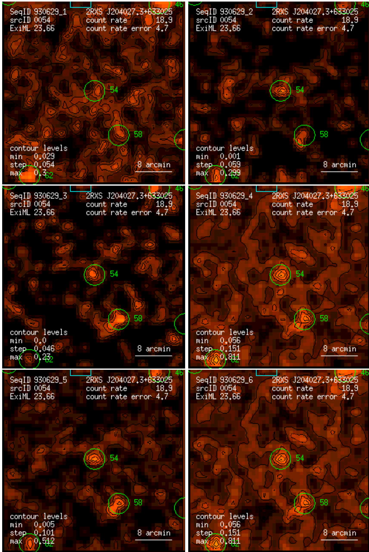
Figure 54: RASS 930629: detection 0054: band rate images, Gaussian filter: (1) PSPC channels 11 – 41, (2) 52 – 90, (3) 91 – 201, (4) 11 – 235, (5) 52 – 201, (6) 11 – 201. Broad band rates in counts/ks. Band rate contour levels in counts/ks/arcmin 2 .
