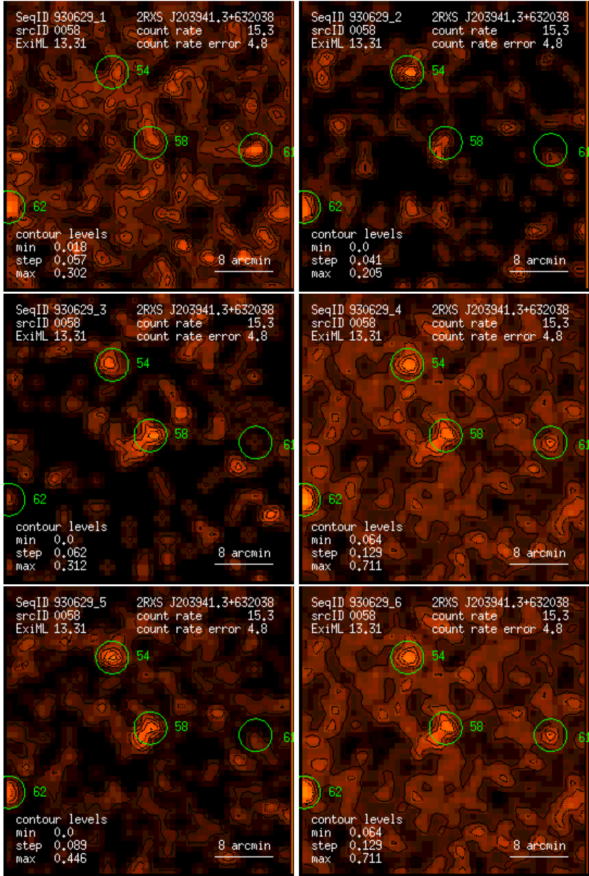
Figure 58: RASS 930629: detection 0058: band rate images, Gaussian filter: (1) PSPC channels 11 – 41, (2) 52 – 90, (3) 91 – 201, (4) 11 – 235, (5) 52 – 201, (6) 11 – 201. Broad band rates in counts/ks. Band rate contour levels in counts/ks/arcmin 2 .
