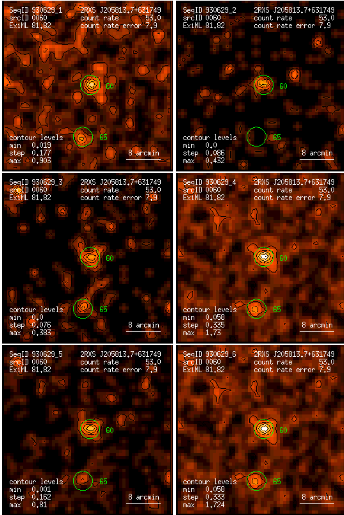
Figure 60: RASS 930629: detection 0060: band rate images, Gaussian filter: (1) PSPC channels 11 – 41, (2) 52 – 90, (3) 91 – 201, (4) 11 – 235, (5) 52 – 201, (6) 11 – 201. Broad band rates in counts/ks. Band rate contour levels in counts/ks/arcmin 2 .
